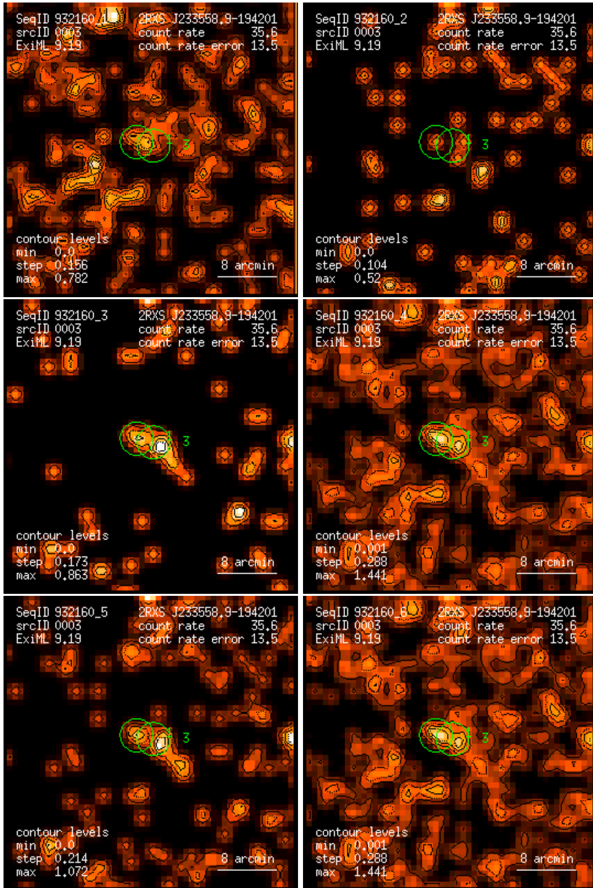
Figure 3: RASS 932160: detection 0003: band rate images, Gaussian filter: (1) PSPC channels 11 – 41, (2) 52 – 90, (3) 91 – 201, (4) 11 – 235, (5) 52 – 201, (6) 11 – 201. Broad band rates in counts/ks. Band rate contour levels in counts/ks/arcmin 2 .
