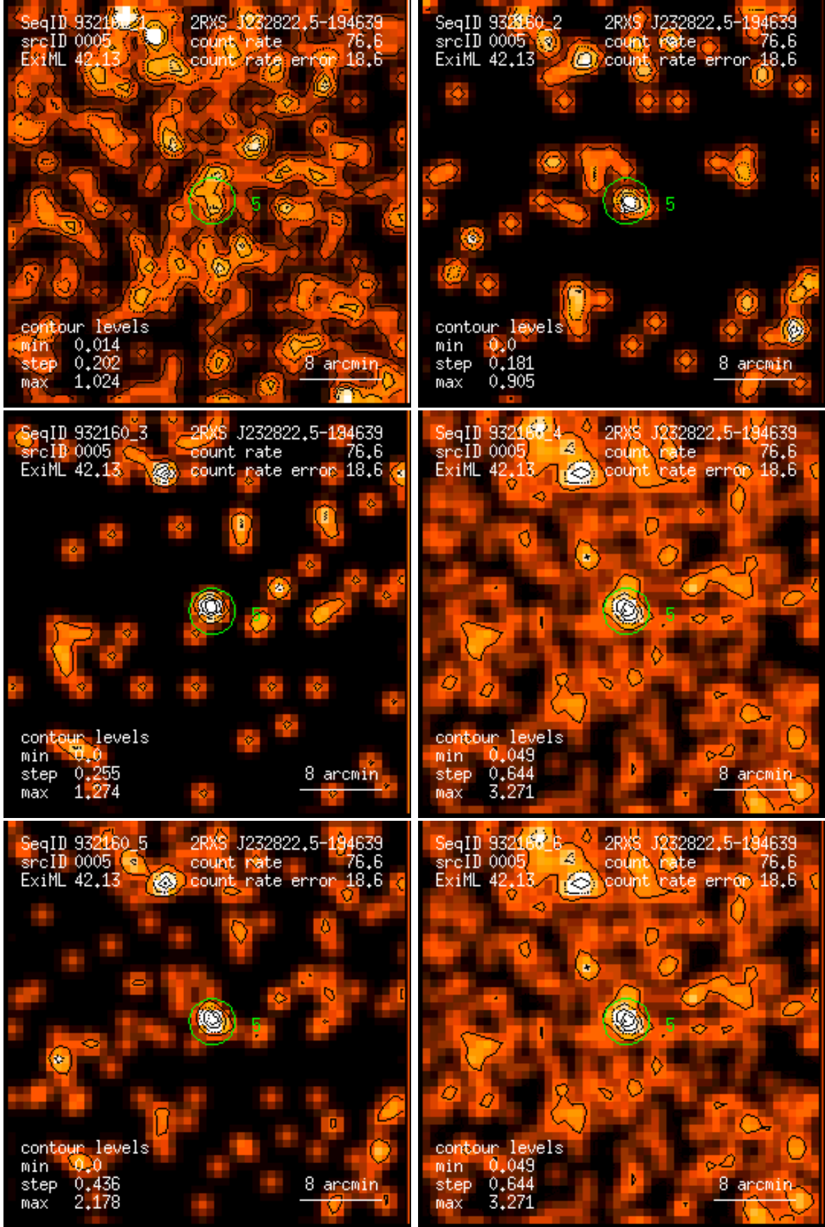
Figure 5: RASS 932160: detection 0005: band rate images, Gaussian filter: (1) PSPC channels 11 – 41, (2) 52 – 90, (3) 91 – 201, (4) 11 – 235, (5) 52 – 201, (6) 11 – 201. Broad band rates in counts/ks. Band rate contour levels in counts/ks/arcmin 2 .
