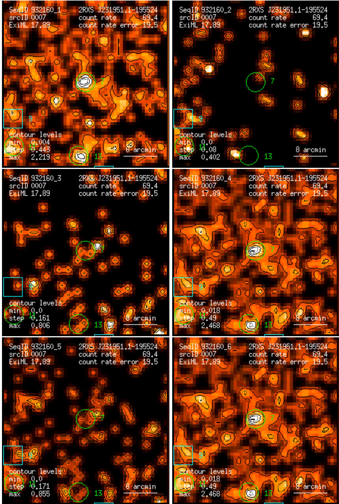
Figure 7: RASS 932160: detection 0007: band rate images, Gaussian filter: (1) PSPC channels 11 – 41, (2) 52 – 90, (3) 91 – 201, (4) 11 – 235, (5) 52 – 201, (6) 11 – 201. Broad band rates in counts/ks. Band rate contour levels in counts/ks/arcmin 2 .
