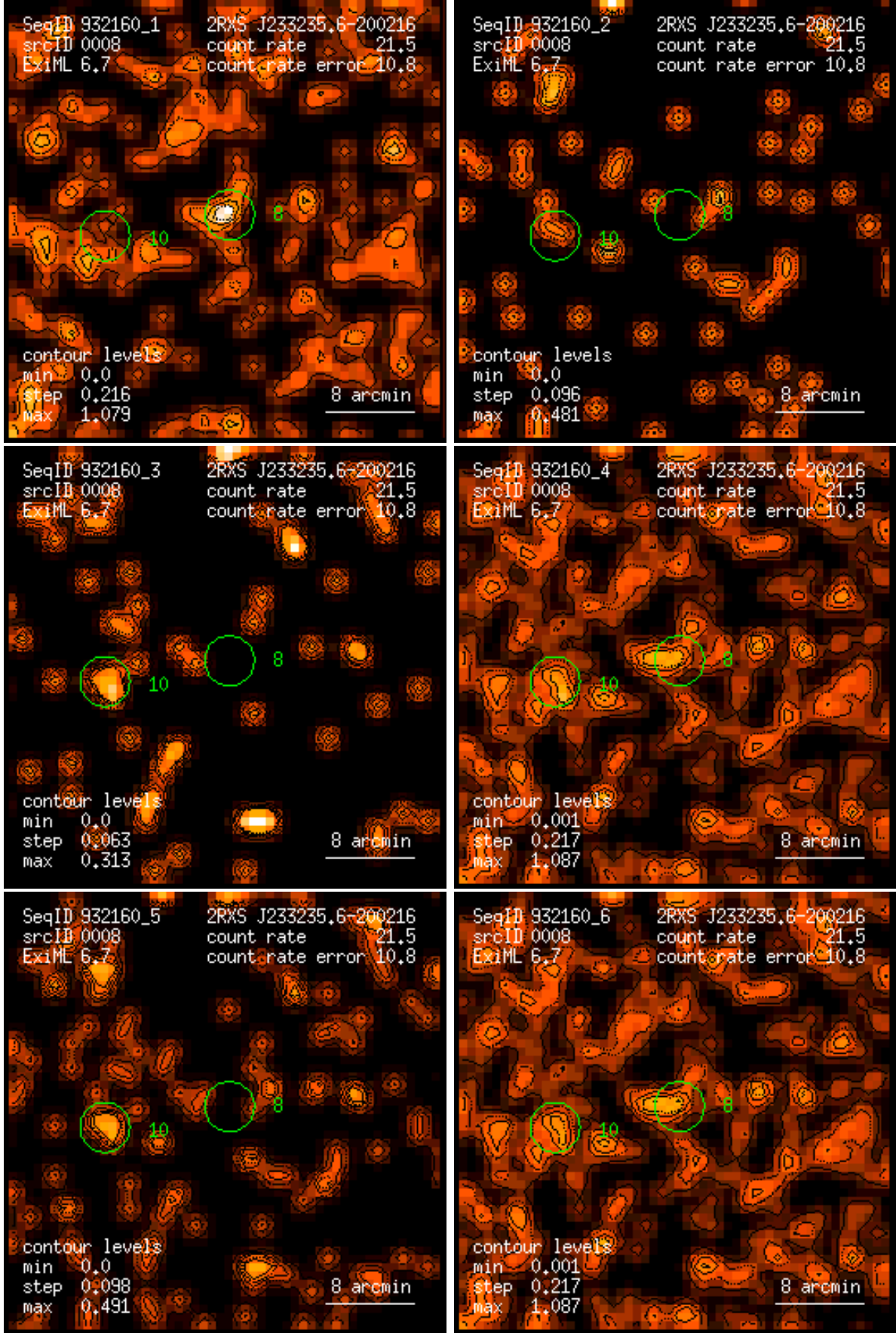
Figure 8: RASS 932160: detection 0008: band rate images, Gaussian filter: (1) PSPC channels 11 – 41, (2) 52 – 90, (3) 91 – 201, (4) 11 – 235, (5) 52 – 201, (6) 11 – 201. Broad band rates in counts/ks. Band rate contour levels in counts/ks/arcmin 2 .
