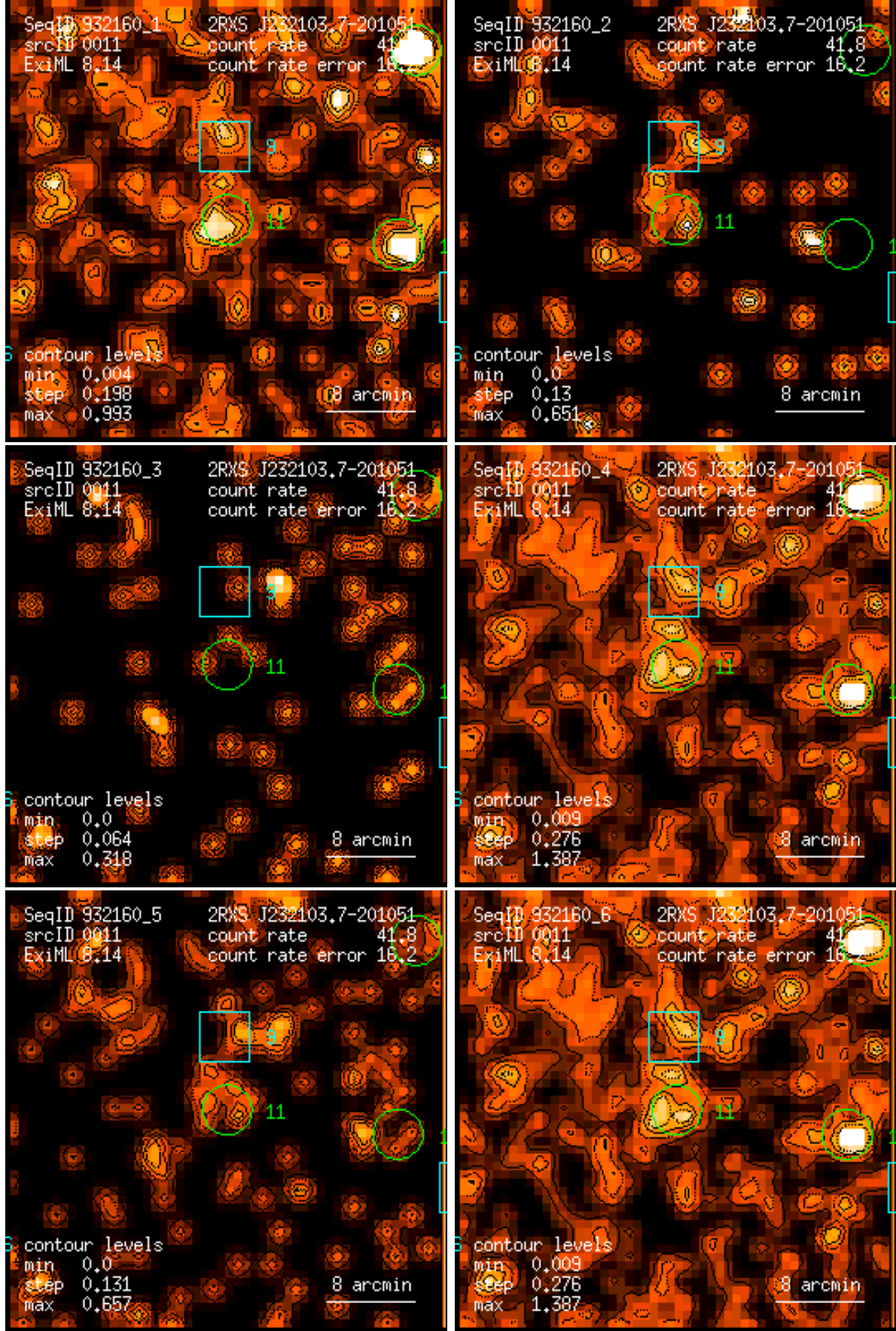
Figure 11: RASS 932160: detection 0011: band rate images, Gaussian filter: (1) PSPC channels 11 – 41, (2) 52 – 90, (3) 91 – 201, (4) 11 – 235, (5) 52 – 201, (6) 11 – 201. Broad band rates in counts/ks. Band rate contour levels in counts/ks/arcmin 2 .
