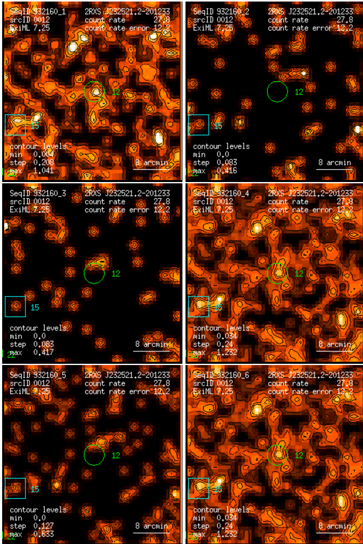
Figure 12: RASS 932160: detection 0012: band rate images, Gaussian filter: (1) PSPC channels 11 – 41, (2) 52 – 90, (3) 91 – 201, (4) 11 – 235, (5) 52 – 201, (6) 11 – 201. Broad band rates in counts/ks. Band rate contour levels in counts/ks/arcmin 2 .
