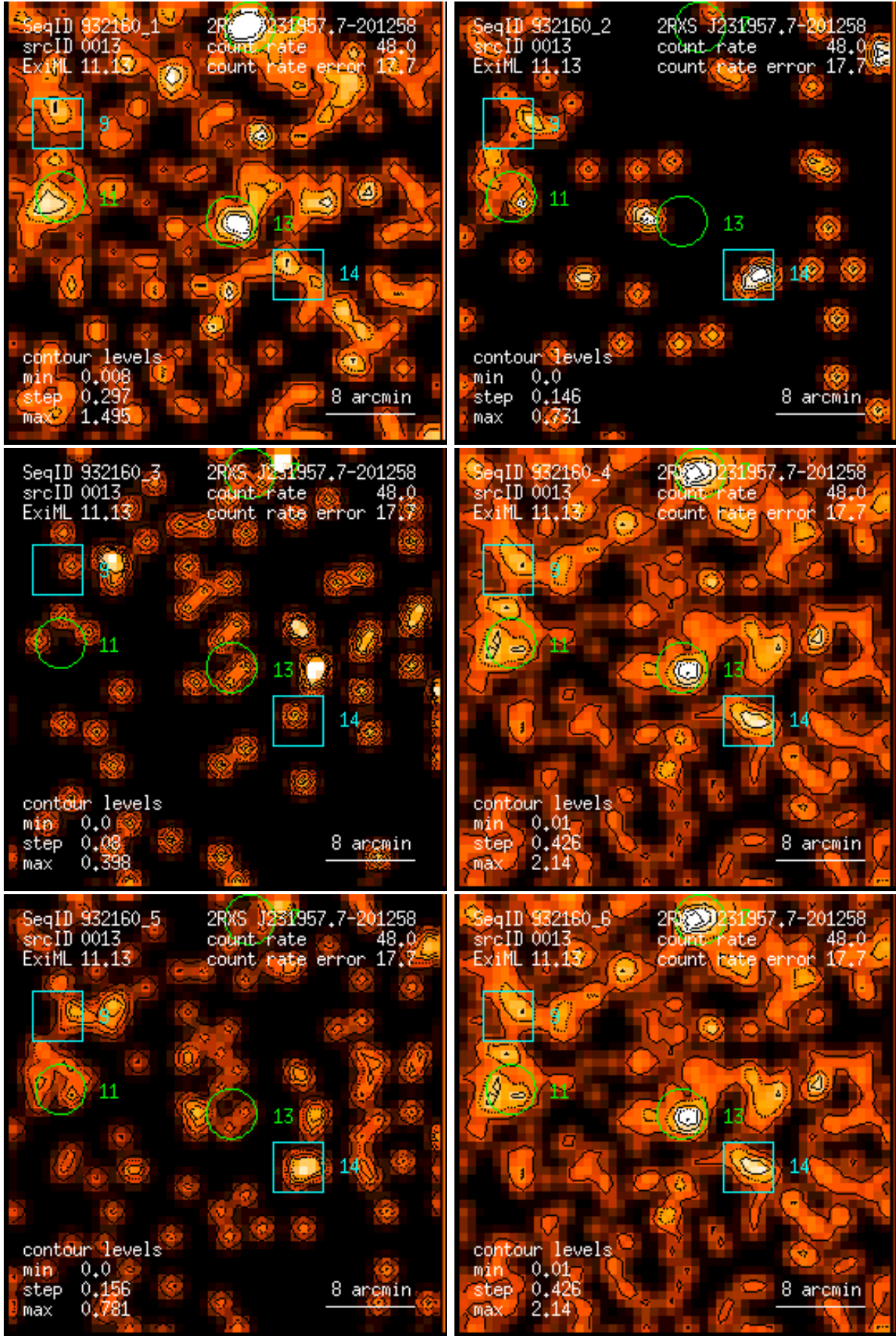
Figure 13: RASS 932160: detection 0013: band rate images, Gaussian filter: (1) PSPC channels 11 – 41, (2) 52 – 90, (3) 91 – 201, (4) 11 – 235, (5) 52 – 201, (6) 11 – 201. Broad band rates in counts/ks. Band rate contour levels in counts/ks/arcmin 2 .
