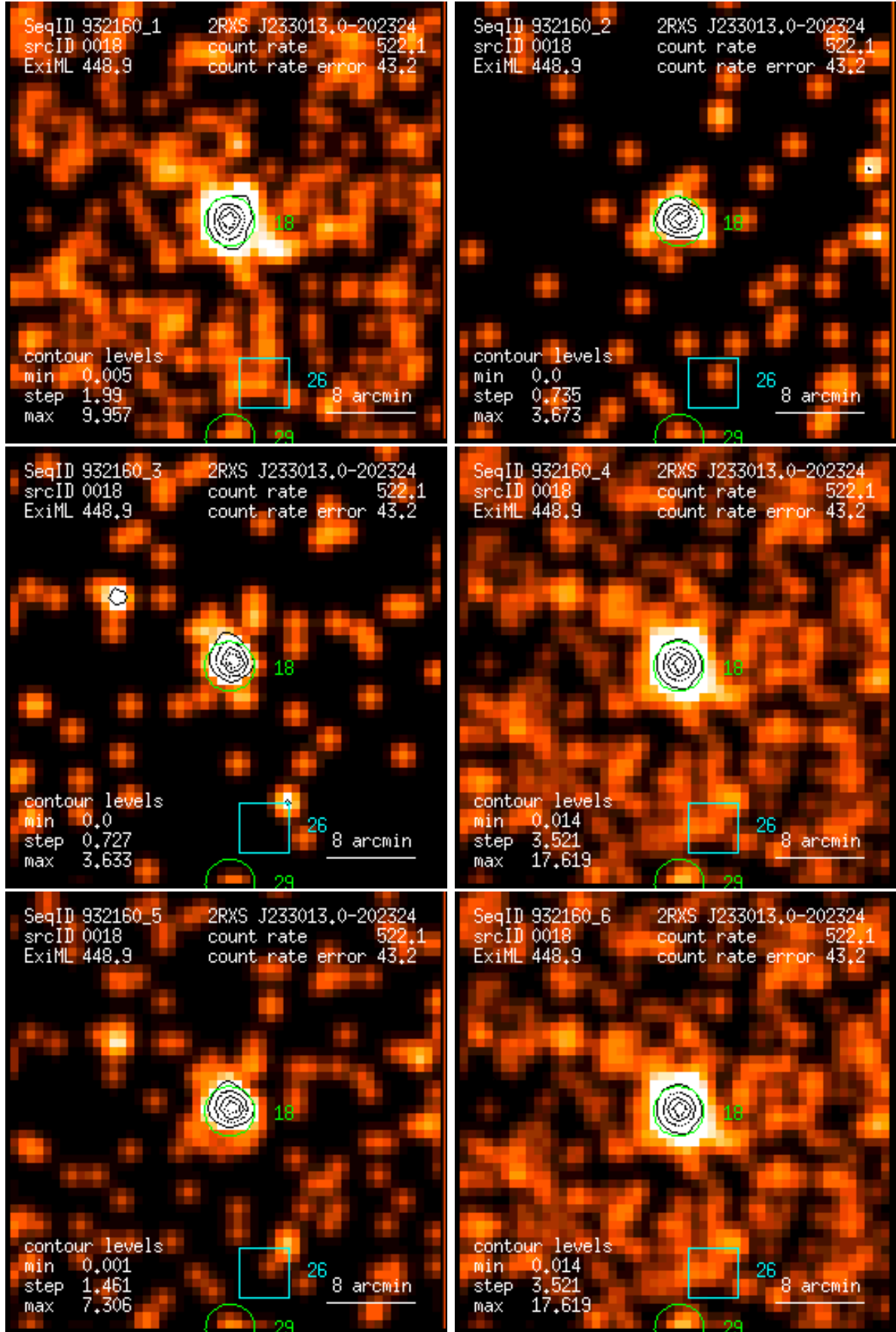
Figure 18: RASS 932160: detection 0018: band rate images, Gaussian filter: (1) PSPC channels 11 – 41, (2) 52 – 90, (3) 91 – 201, (4) 11 – 235, (5) 52 – 201, (6) 11 – 201. Broad band rates in counts/ks. Band rate contour levels in counts/ks/arcmin 2 .
