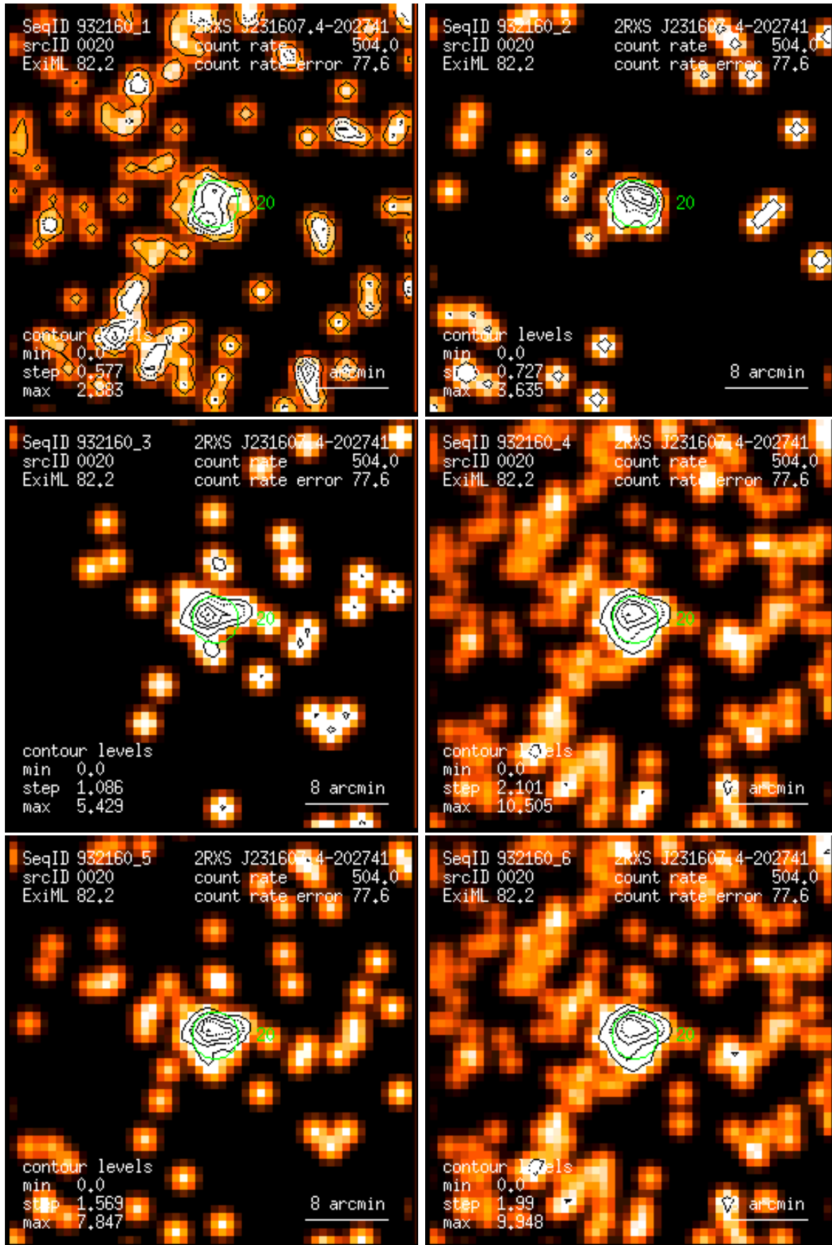
Figure 20: RASS 932160: detection 0020: band rate images, Gaussian filter: (1) PSPC channels 11 – 41, (2) 52 – 90, (3) 91 – 201, (4) 11 – 235, (5) 52 – 201, (6) 11 – 201. Broad band rates in counts/ks. Band rate contour levels in counts/ks/arcmin 2 .
