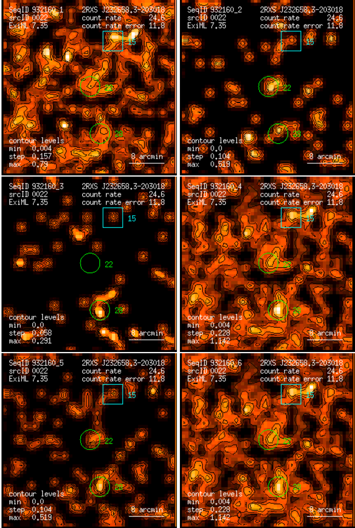
Figure 22: RASS 932160: detection 0022: band rate images, Gaussian filter: (1) PSPC channels 11 – 41, (2) 52 – 90, (3) 91 – 201, (4) 11 – 235, (5) 52 – 201, (6) 11 – 201. Broad band rates in counts/ks. Band rate contour levels in counts/ks/arcmin 2 .
