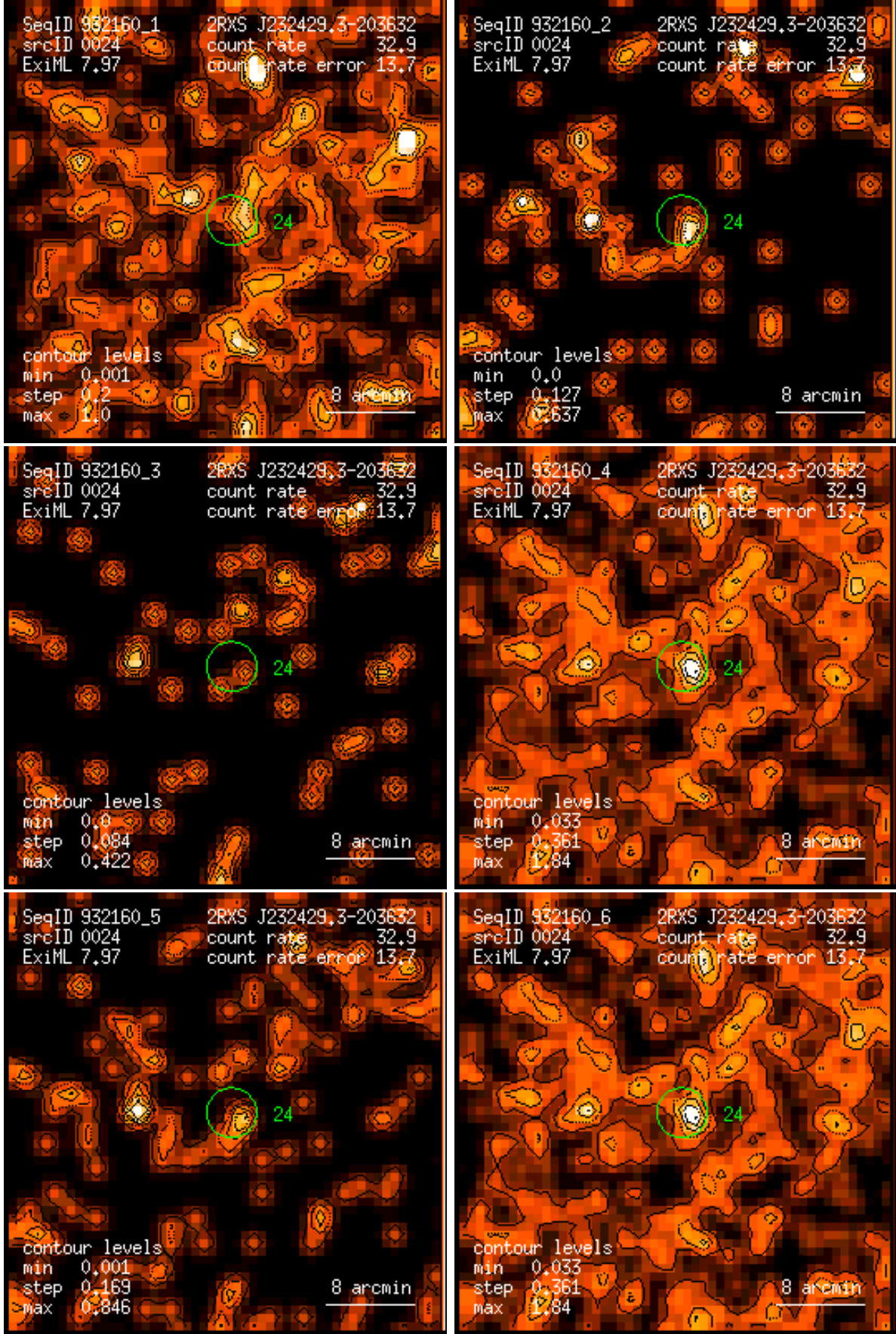
Figure 24: RASS 932160: detection 0024: band rate images, Gaussian filter: (1) PSPC channels 11 – 41, (2) 52 – 90, (3) 91 – 201, (4) 11 – 235, (5) 52 – 201, (6) 11 – 201. Broad band rates in counts/ks. Band rate contour levels in counts/ks/arcmin 2 .
