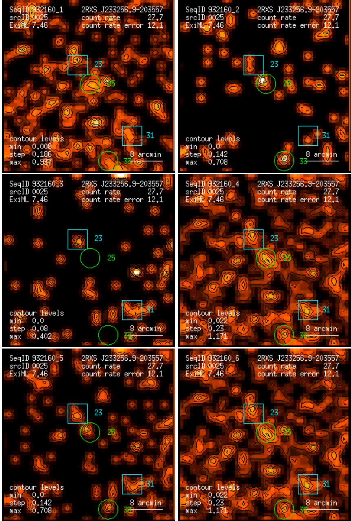
Figure 25: RASS 932160: detection 0025: band rate images, Gaussian filter: (1) PSPC channels 11 – 41, (2) 52 – 90, (3) 91 – 201, (4) 11 – 235, (5) 52 – 201, (6) 11 – 201. Broad band rates in counts/ks. Band rate contour levels in counts/ks/arcmin 2 .
