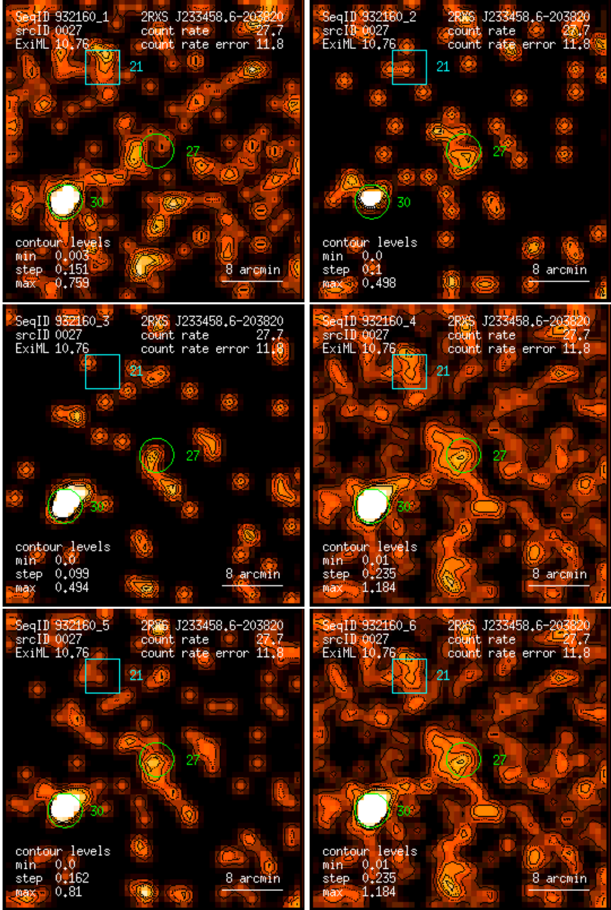
Figure 27: RASS 932160: detection 0027: band rate images, Gaussian filter: (1) PSPC channels 11 – 41, (2) 52 – 90, (3) 91 – 201, (4) 11 – 235, (5) 52 – 201, (6) 11 – 201. Broad band rates in counts/ks. Band rate contour levels in counts/ks/arcmin 2 .
