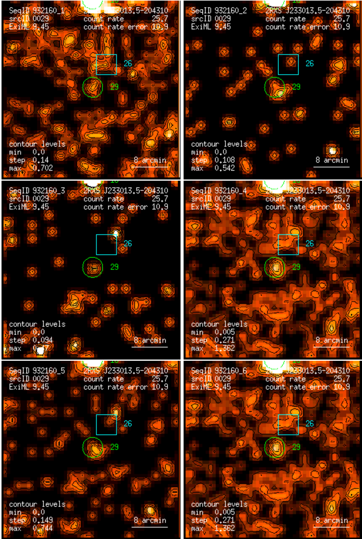
Figure 29: RASS 932160: detection 0029: band rate images, Gaussian filter: (1) PSPC channels 11 – 41, (2) 52 – 90, (3) 91 – 201, (4) 11 – 235, (5) 52 – 201, (6) 11 – 201. Broad band rates in counts/ks. Band rate contour levels in counts/ks/arcmin 2 .
