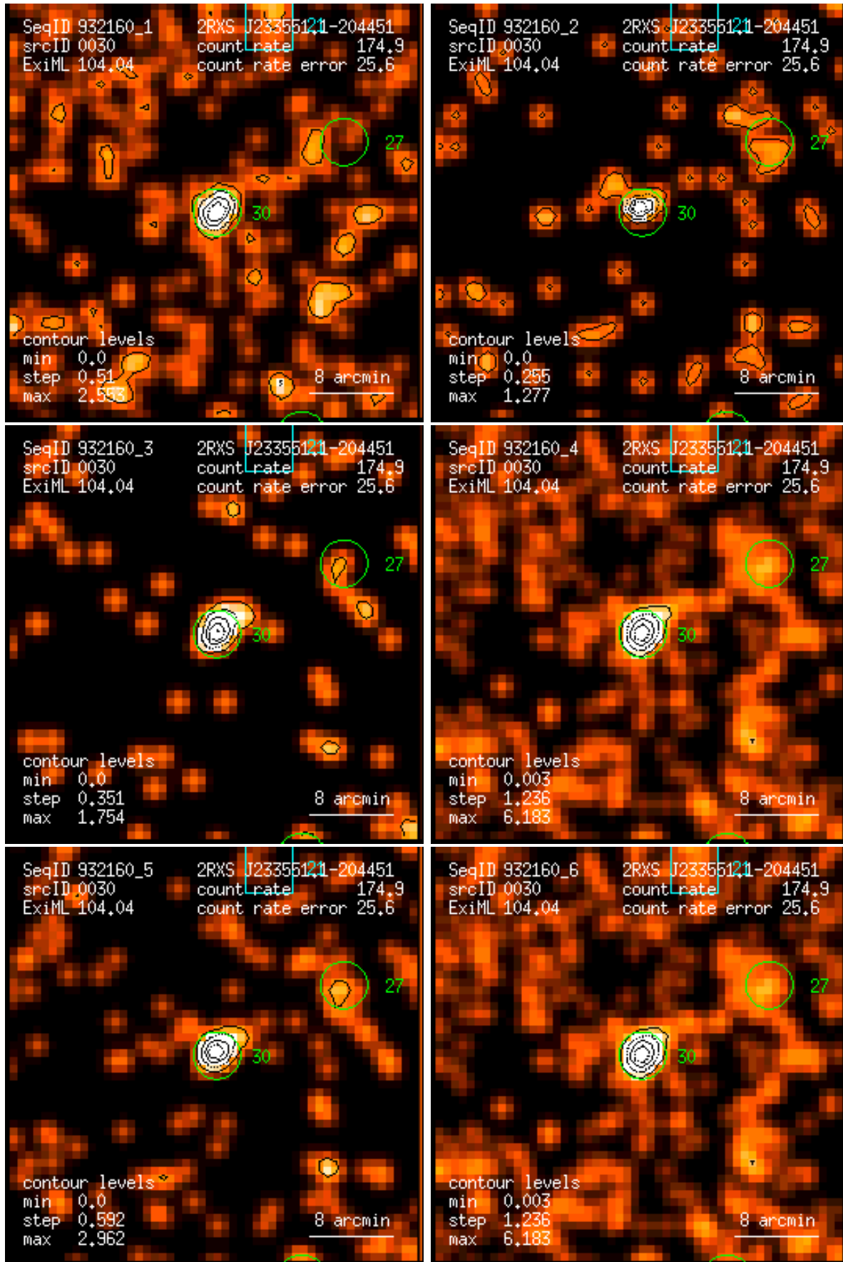
Figure 30: RASS 932160: detection 0030: band rate images, Gaussian filter: (1) PSPC channels 11 – 41, (2) 52 – 90, (3) 91 – 201, (4) 11 – 235, (5) 52 – 201, (6) 11 – 201. Broad band rates in counts/ks. Band rate contour levels in counts/ks/arcmin 2 .
