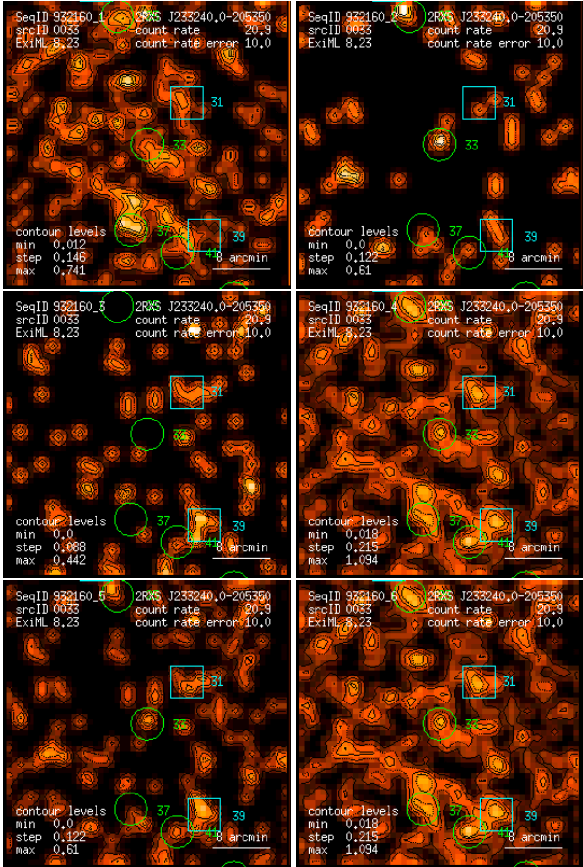
Figure 33: RASS 932160: detection 0033: band rate images, Gaussian filter: (1) PSPC channels 11 – 41, (2) 52 – 90, (3) 91 – 201, (4) 11 – 235, (5) 52 – 201, (6) 11 – 201. Broad band rates in counts/ks. Band rate contour levels in counts/ks/arcmin 2 .
