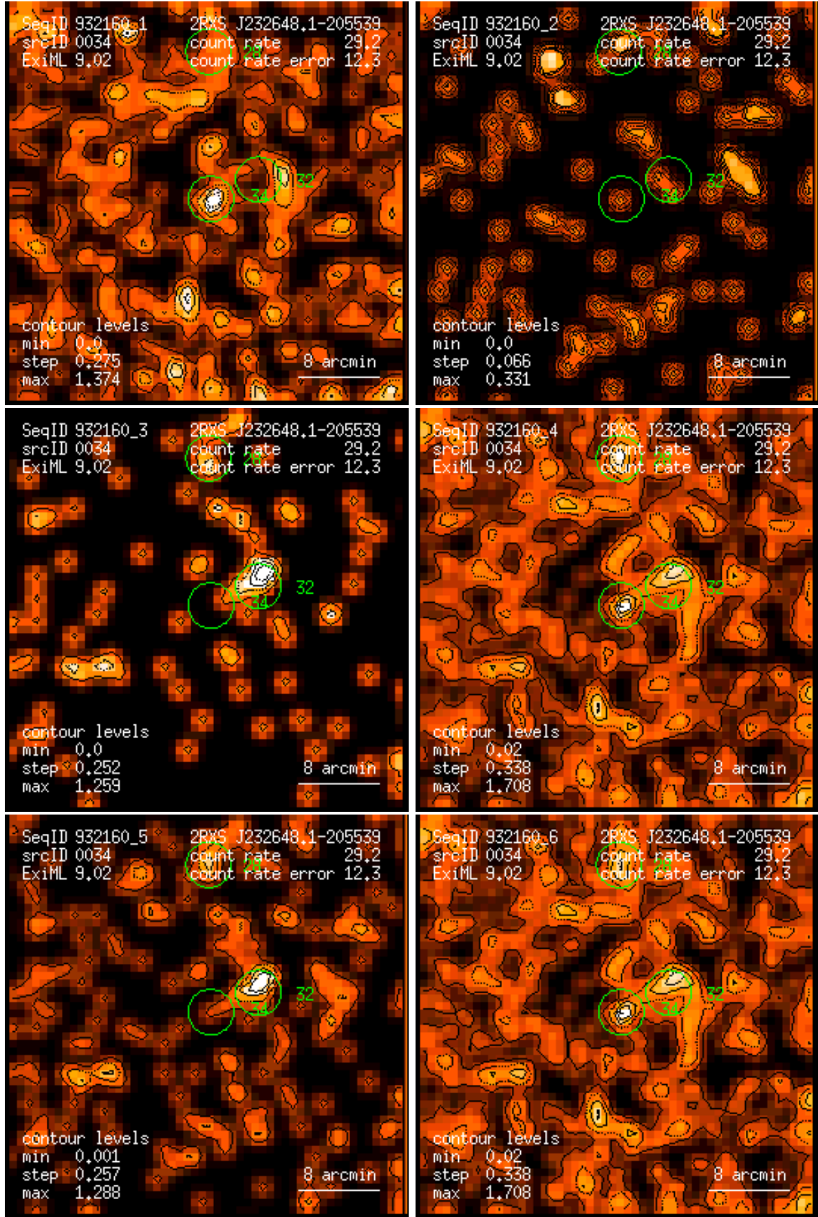
Figure 34: RASS 932160: detection 0034: band rate images, Gaussian filter: (1) PSPC channels 11 – 41, (2) 52 – 90, (3) 91 – 201, (4) 11 – 235, (5) 52 – 201, (6) 11 – 201. Broad band rates in counts/ks. Band rate contour levels in counts/ks/arcmin 2 .
