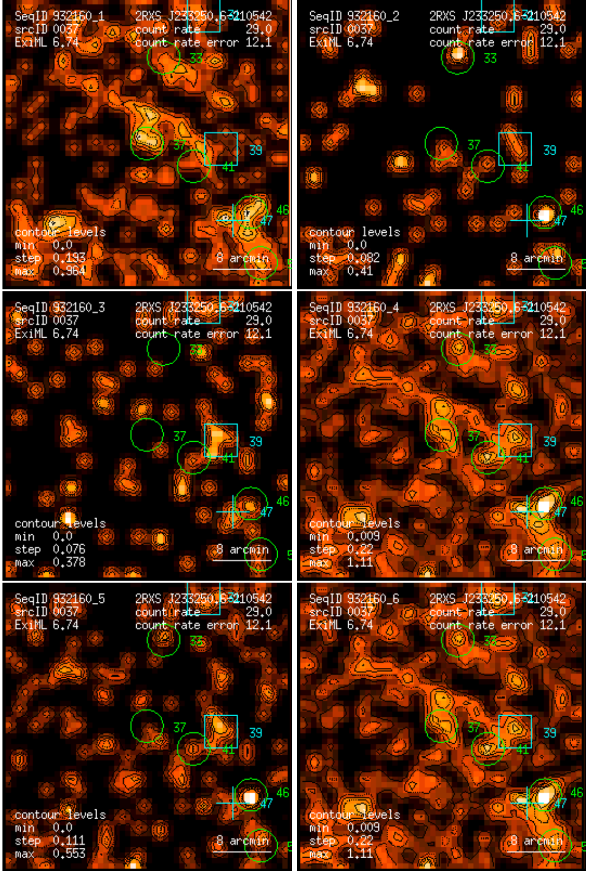
Figure 37: RASS 932160: detection 0037: band rate images, Gaussian filter: (1) PSPC channels 11 – 41, (2) 52 – 90, (3) 91 – 201, (4) 11 – 235, (5) 52 – 201, (6) 11 – 201. Broad band rates in counts/ks. Band rate contour levels in counts/ks/arcmin 2 .
