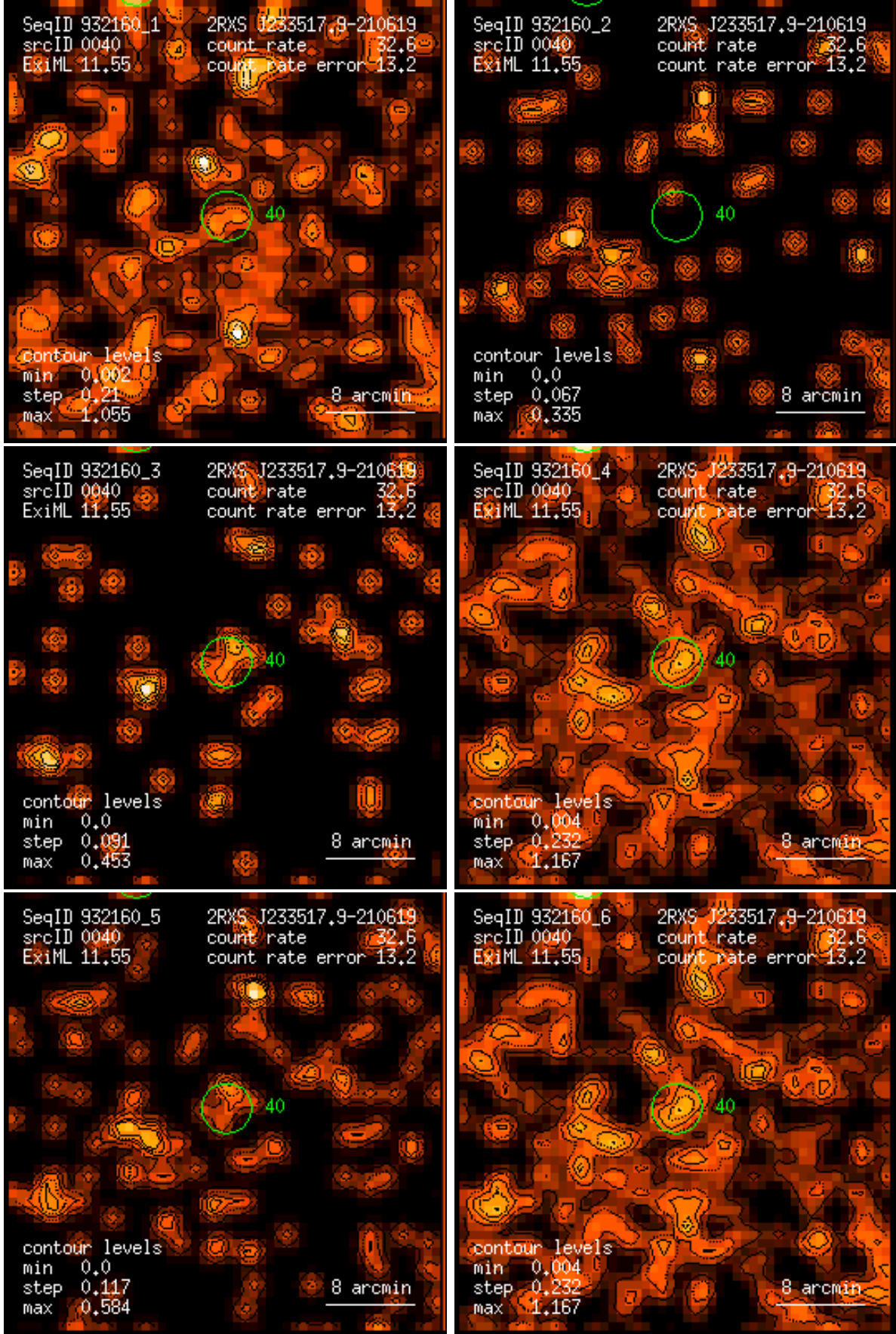
Figure 40: RASS 932160: detection 0040: band rate images, Gaussian filter: (1) PSPC channels 11 – 41, (2) 52 – 90, (3) 91 – 201, (4) 11 – 235, (5) 52 – 201, (6) 11 – 201. Broad band rates in counts/ks. Band rate contour levels in counts/ks/arcmin 2 .
