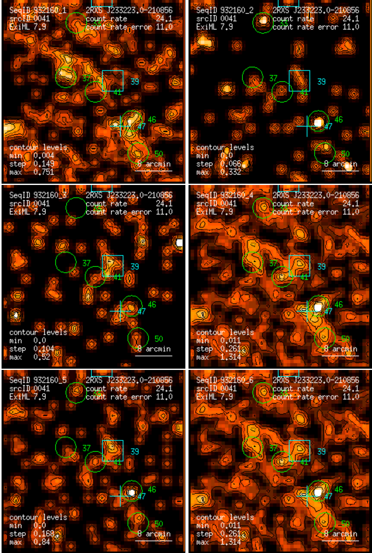
Figure 41: RASS 932160: detection 0041: band rate images, Gaussian filter: (1) PSPC channels 11 – 41, (2) 52 – 90, (3) 91 – 201, (4) 11 – 235, (5) 52 – 201, (6) 11 – 201. Broad band rates in counts/ks. Band rate contour levels in counts/ks/arcmin 2 .
