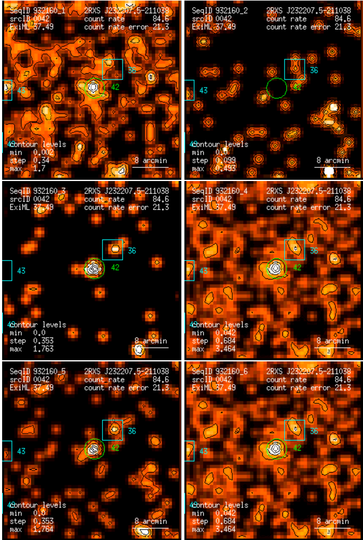
Figure 42: RASS 932160: detection 0042: band rate images, Gaussian filter: (1) PSPC channels 11 – 41, (2) 52 – 90, (3) 91 – 201, (4) 11 – 235, (5) 52 – 201, (6) 11 – 201. Broad band rates in counts/ks. Band rate contour levels in counts/ks/arcmin 2 .
