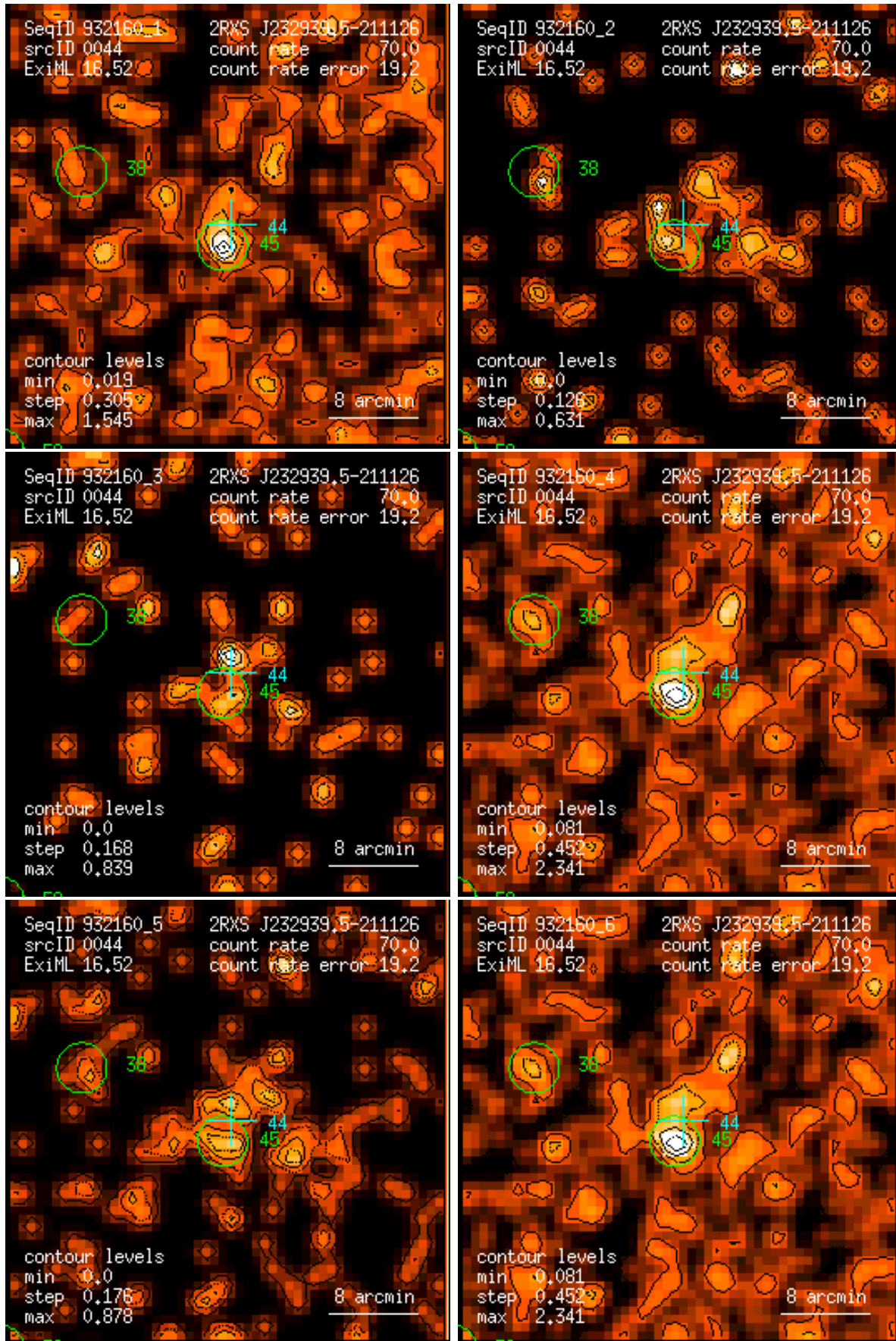
Figure 44: RASS 932160: detection 0044: band rate images, Gaussian filter: (1) PSPC channels 11 – 41, (2) 52 – 90, (3) 91 – 201, (4) 11 – 235, (5) 52 – 201, (6) 11 – 201. Broad band rates in counts/ks. Band rate contour levels in counts/ks/arcmin 2 .
