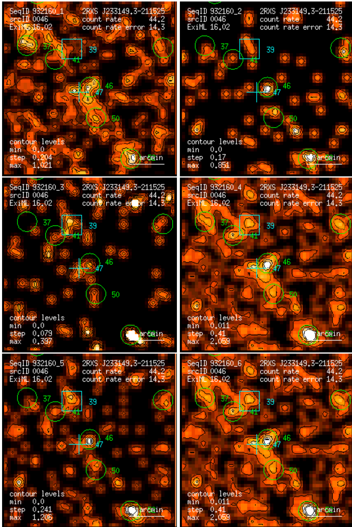
Figure 46: RASS 932160: detection 0046: band rate images, Gaussian filter: (1) PSPC channels 11 – 41, (2) 52 – 90, (3) 91 – 201, (4) 11 – 235, (5) 52 – 201, (6) 11 – 201. Broad band rates in counts/ks. Band rate contour levels in counts/ks/arcmin 2 .
