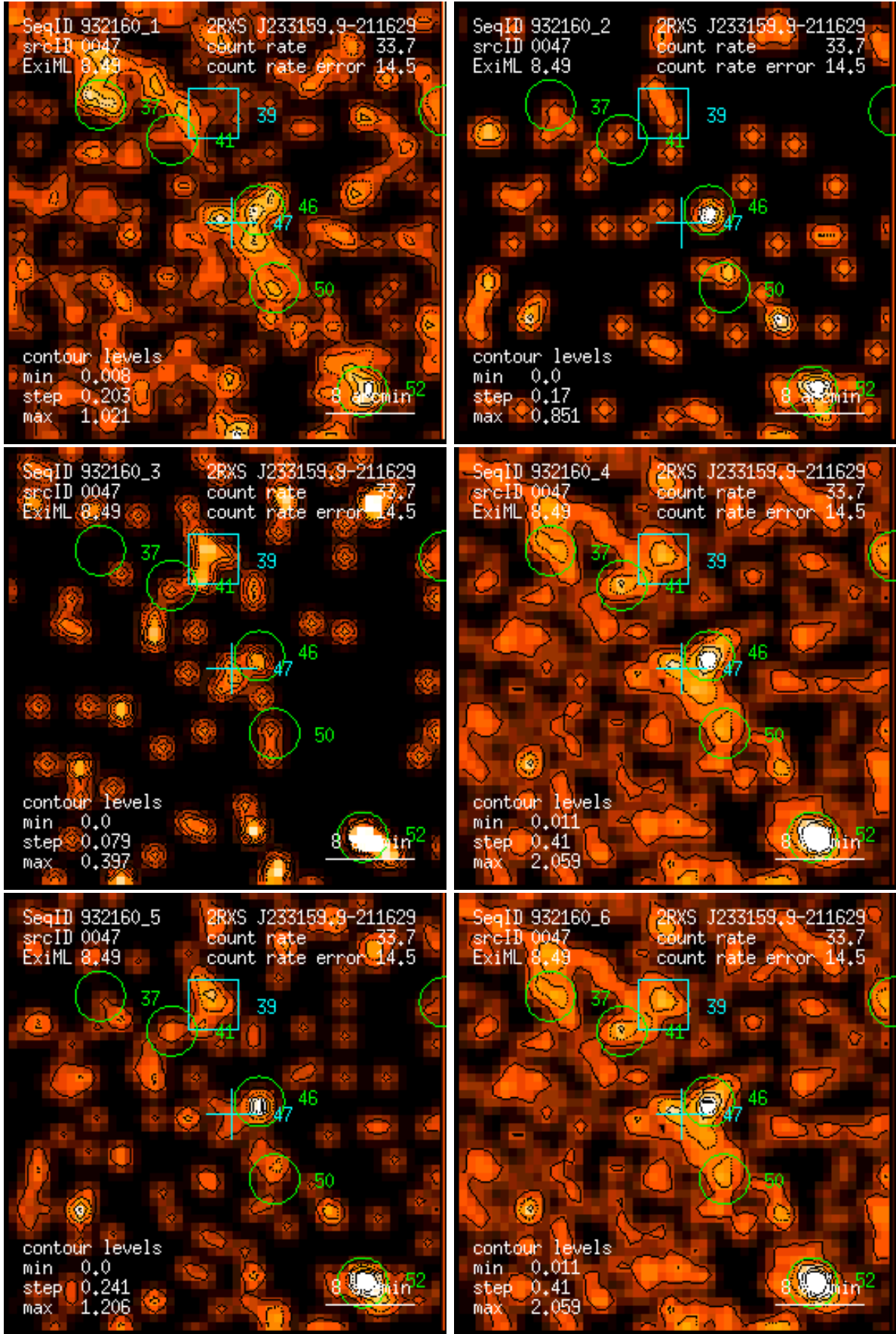
Figure 47: RASS 932160: detection 0047: band rate images, Gaussian filter: (1) PSPC channels 11 – 41, (2) 52 – 90, (3) 91 – 201, (4) 11 – 235, (5) 52 – 201, (6) 11 – 201. Broad band rates in counts/ks. Band rate contour levels in counts/ks/arcmin 2 .
