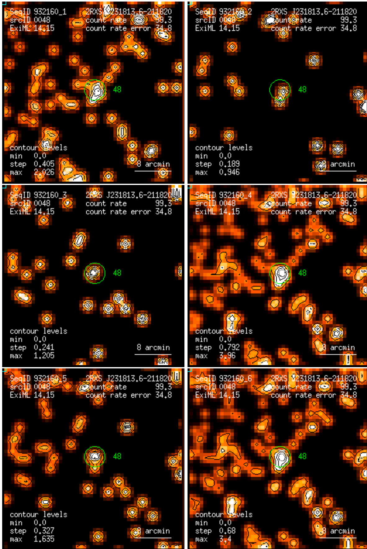
Figure 48: RASS 932160: detection 0048: band rate images, Gaussian filter: (1) PSPC channels 11 – 41, (2) 52 – 90, (3) 91 – 201, (4) 11 – 235, (5) 52 – 201, (6) 11 – 201. Broad band rates in counts/ks. Band rate contour levels in counts/ks/arcmin 2 .
