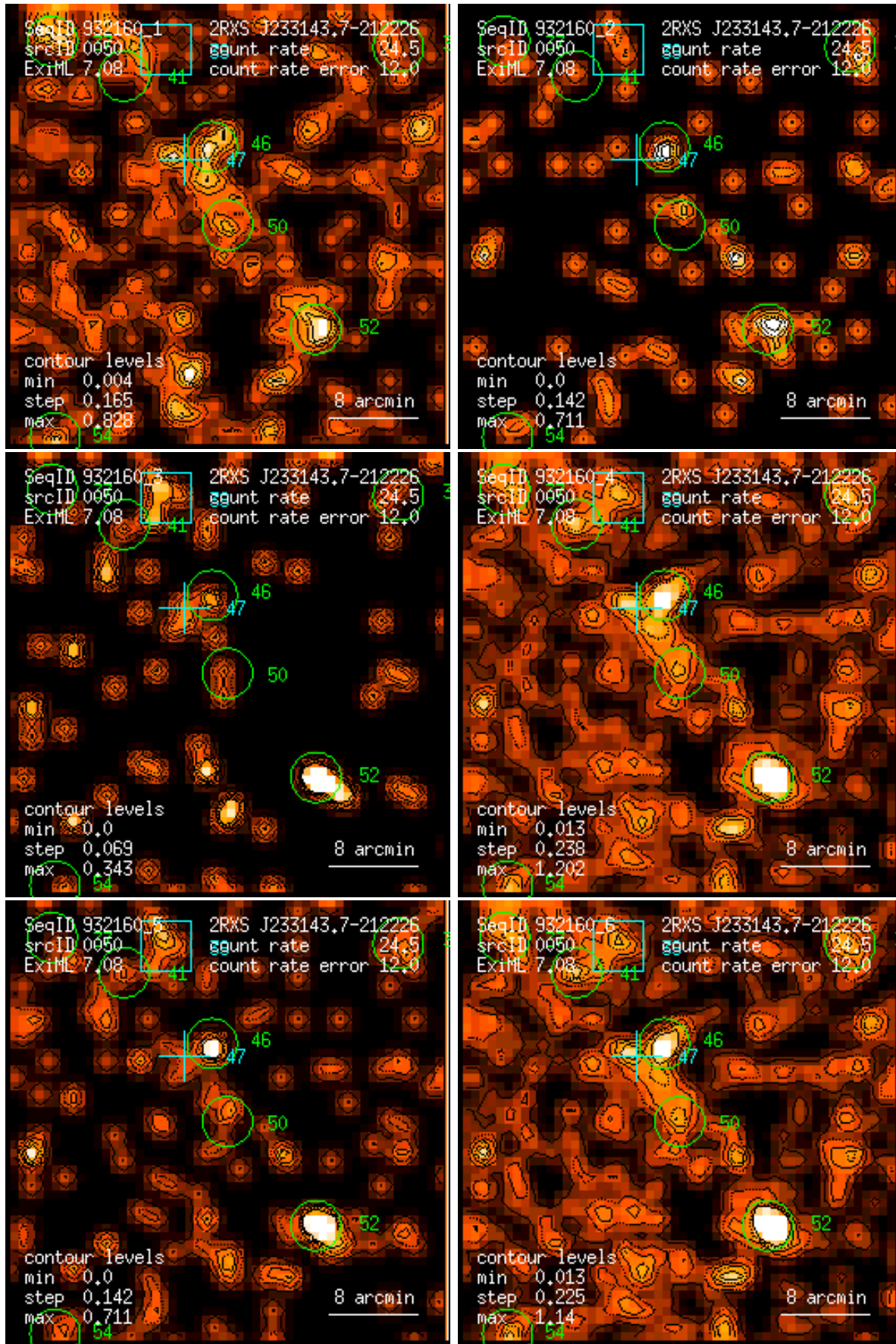
Figure 50: RASS 932160: detection 0050: band rate images, Gaussian filter: (1) PSPC channels 11 – 41, (2) 52 – 90, (3) 91 – 201, (4) 11 – 235, (5) 52 – 201, (6) 11 – 201. Broad band rates in counts/ks. Band rate contour levels in counts/ks/arcmin 2 .
