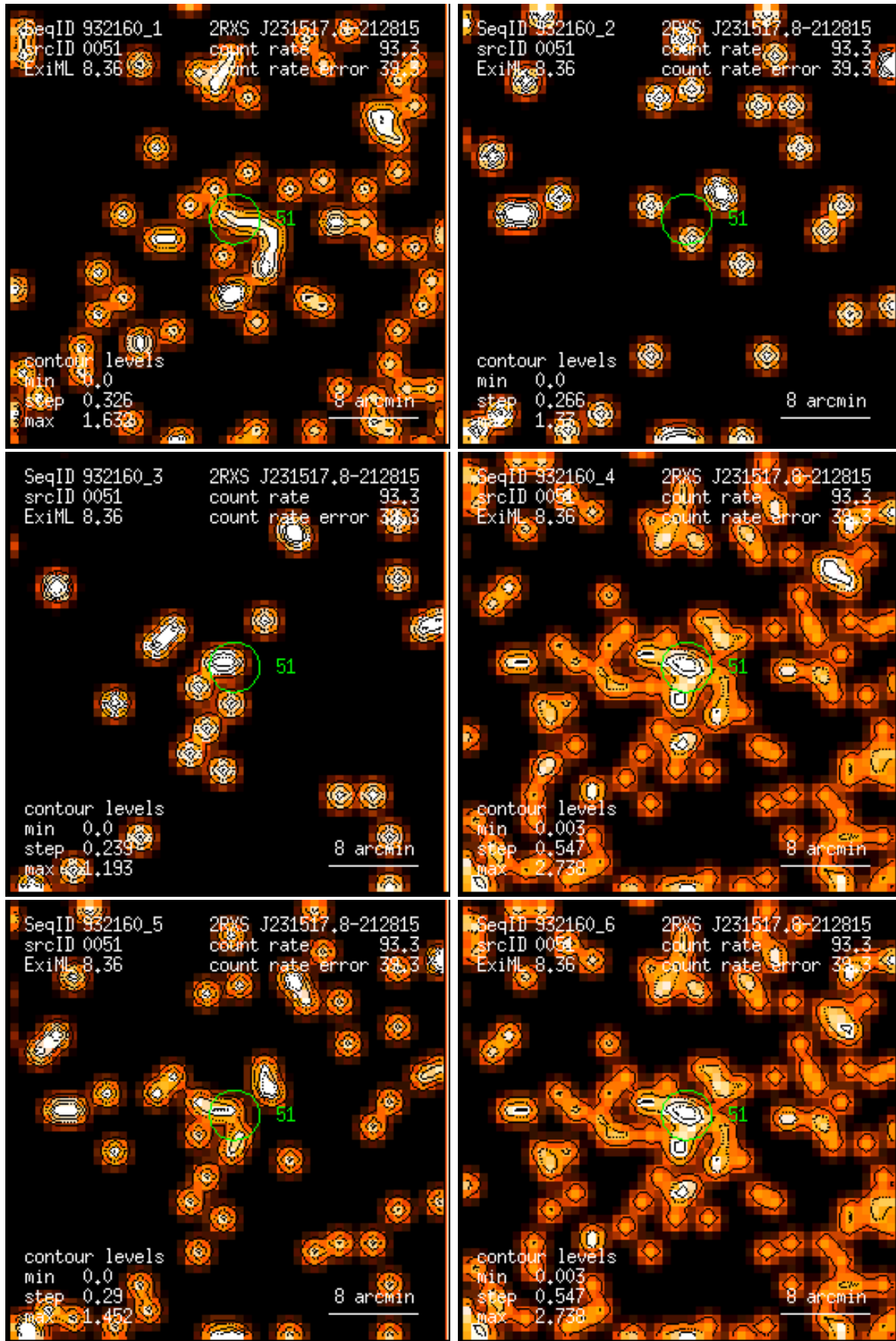
Figure 51: RASS 932160: detection 0051: band rate images, Gaussian filter: (1) PSPC channels 11 – 41, (2) 52 – 90, (3) 91 – 201, (4) 11 – 235, (5) 52 – 201, (6) 11 – 201. Broad band rates in counts/ks. Band rate contour levels in counts/ks/arcmin 2 .
