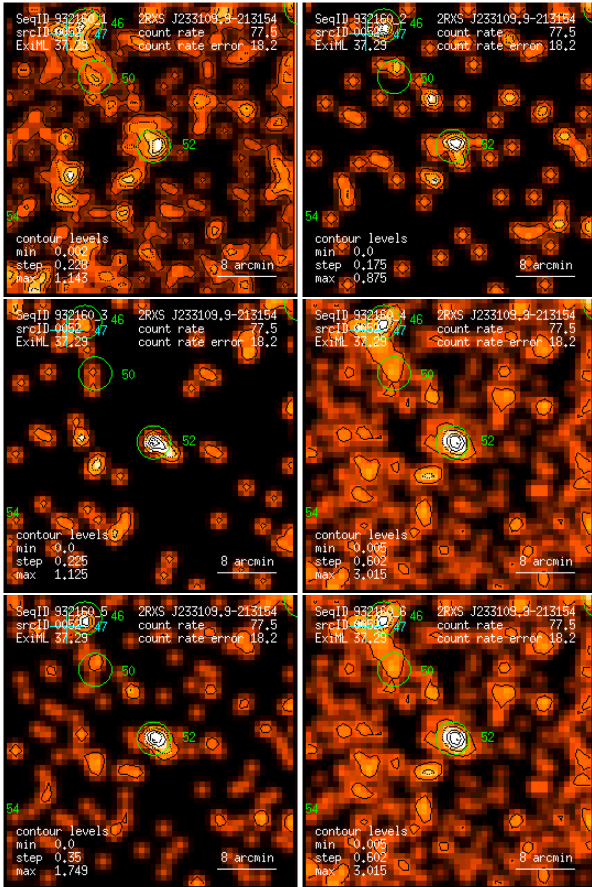
Figure 52: RASS 932160: detection 0052: band rate images, Gaussian filter: (1) PSPC channels 11 – 41, (2) 52 – 90, (3) 91 – 201, (4) 11 – 235, (5) 52 – 201, (6) 11 – 201. Broad band rates in counts/ks. Band rate contour levels in counts/ks/arcmin 2 .
