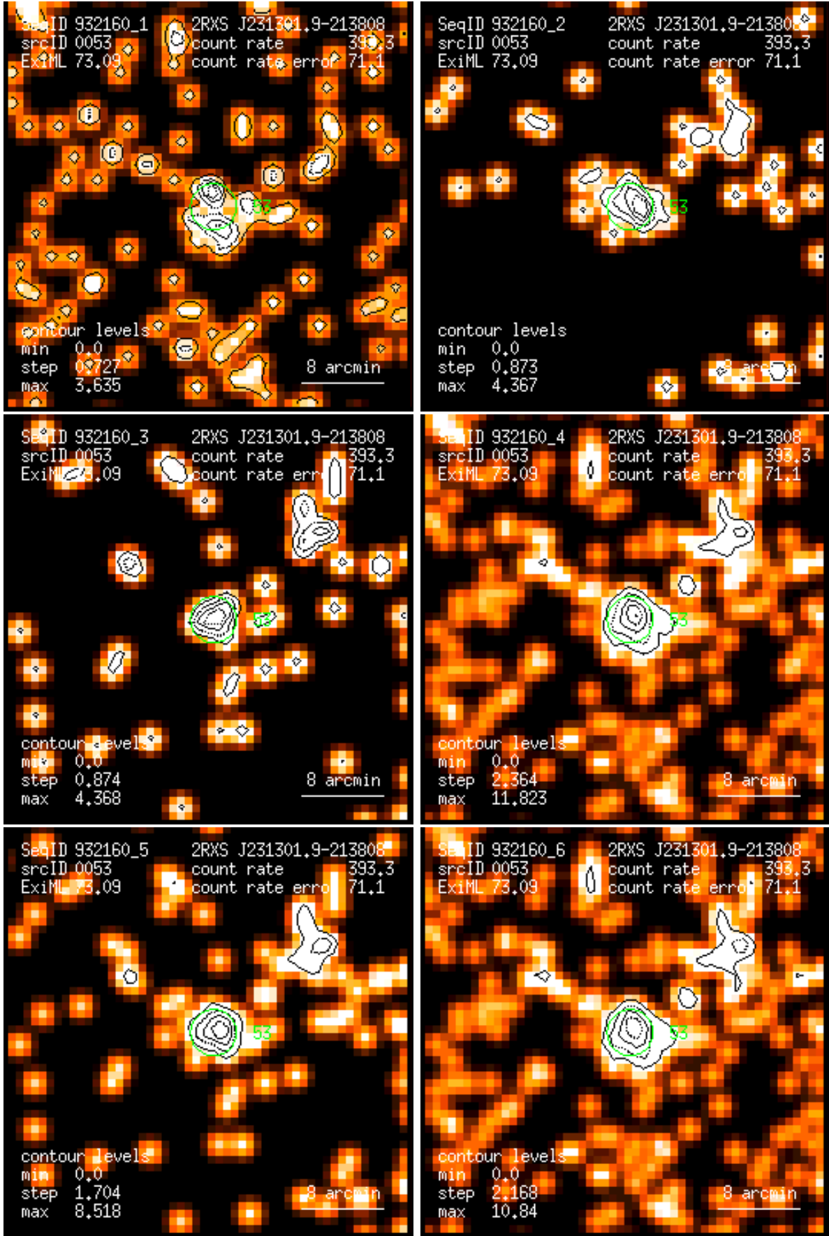
Figure 53: RASS 932160: detection 0053: band rate images, Gaussian filter: (1) PSPC channels 11 – 41, (2) 52 – 90, (3) 91 – 201, (4) 11 – 235, (5) 52 – 201, (6) 11 – 201. Broad band rates in counts/ks. Band rate contour levels in counts/ks/arcmin 2 .
