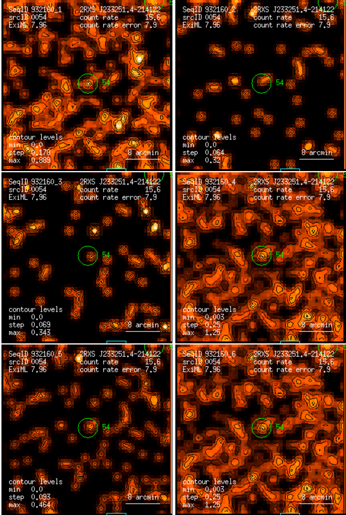
Figure 54: RASS 932160: detection 0054: band rate images, Gaussian filter: (1) PSPC channels 11 – 41, (2) 52 – 90, (3) 91 – 201, (4) 11 – 235, (5) 52 – 201, (6) 11 – 201. Broad band rates in counts/ks. Band rate contour levels in counts/ks/arcmin 2 .
