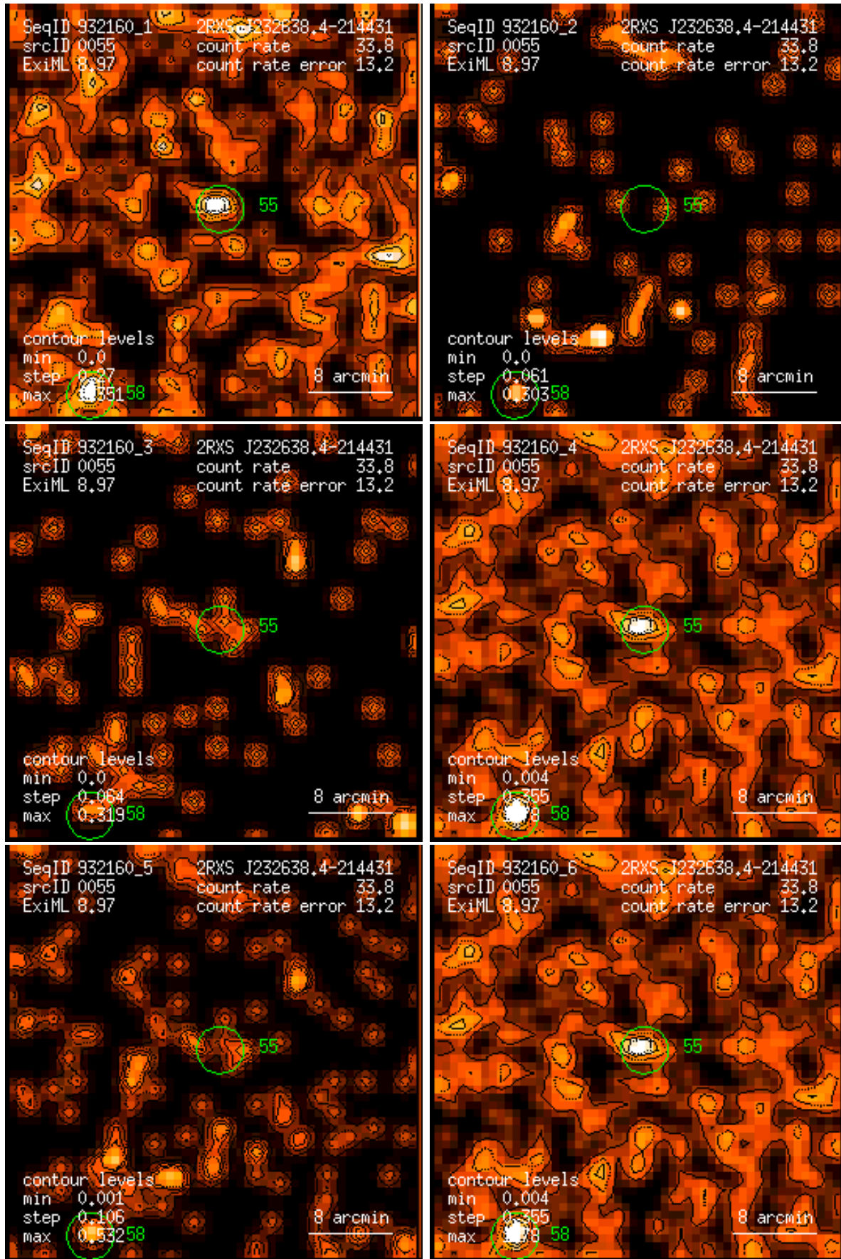
Figure 55: RASS 932160: detection 0055: band rate images, Gaussian filter: (1) PSPC channels 11 – 41, (2) 52 – 90, (3) 91 – 201, (4) 11 – 235, (5) 52 – 201, (6) 11 – 201. Broad band rates in counts/ks. Band rate contour levels in counts/ks/arcmin 2 .
