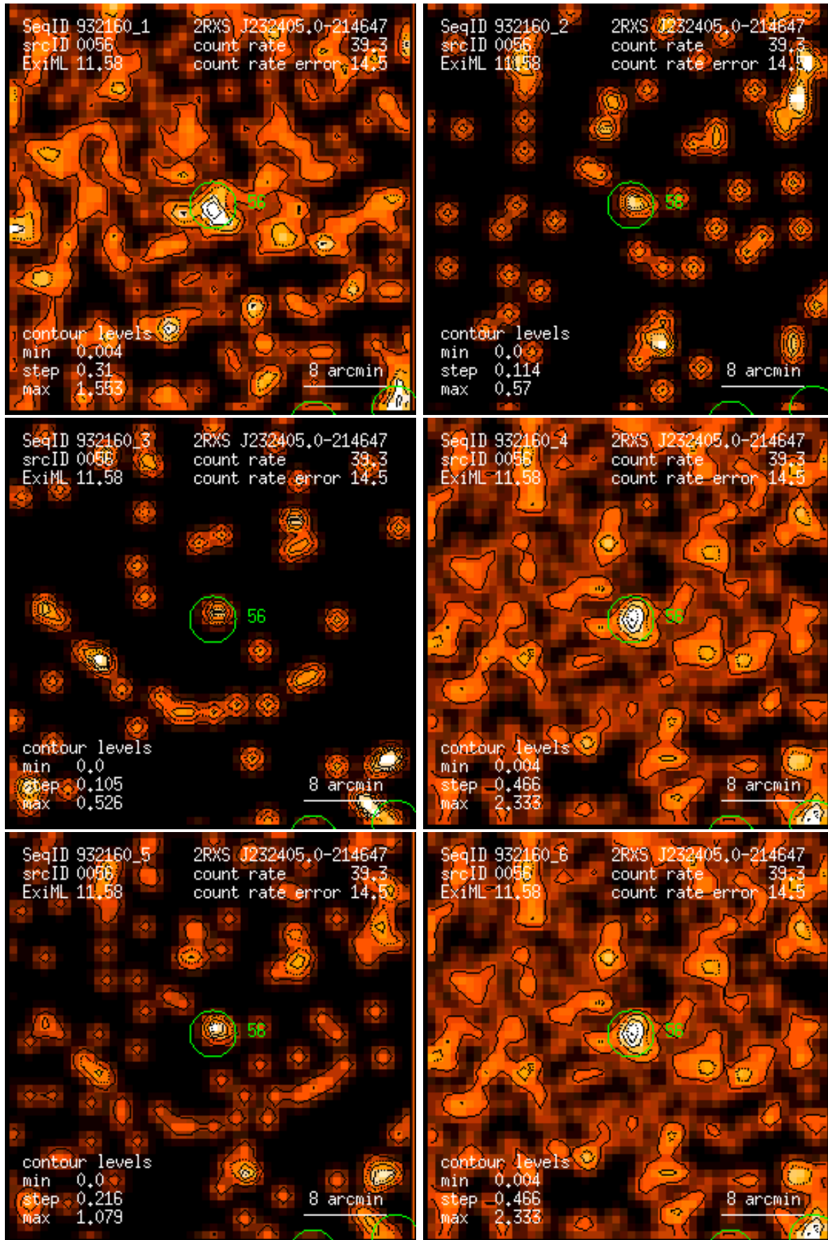
Figure 56: RASS 932160: detection 0056: band rate images, Gaussian filter: (1) PSPC channels 11 – 41, (2) 52 – 90, (3) 91 – 201, (4) 11 – 235, (5) 52 – 201, (6) 11 – 201. Broad band rates in counts/ks. Band rate contour levels in counts/ks/arcmin 2 .
