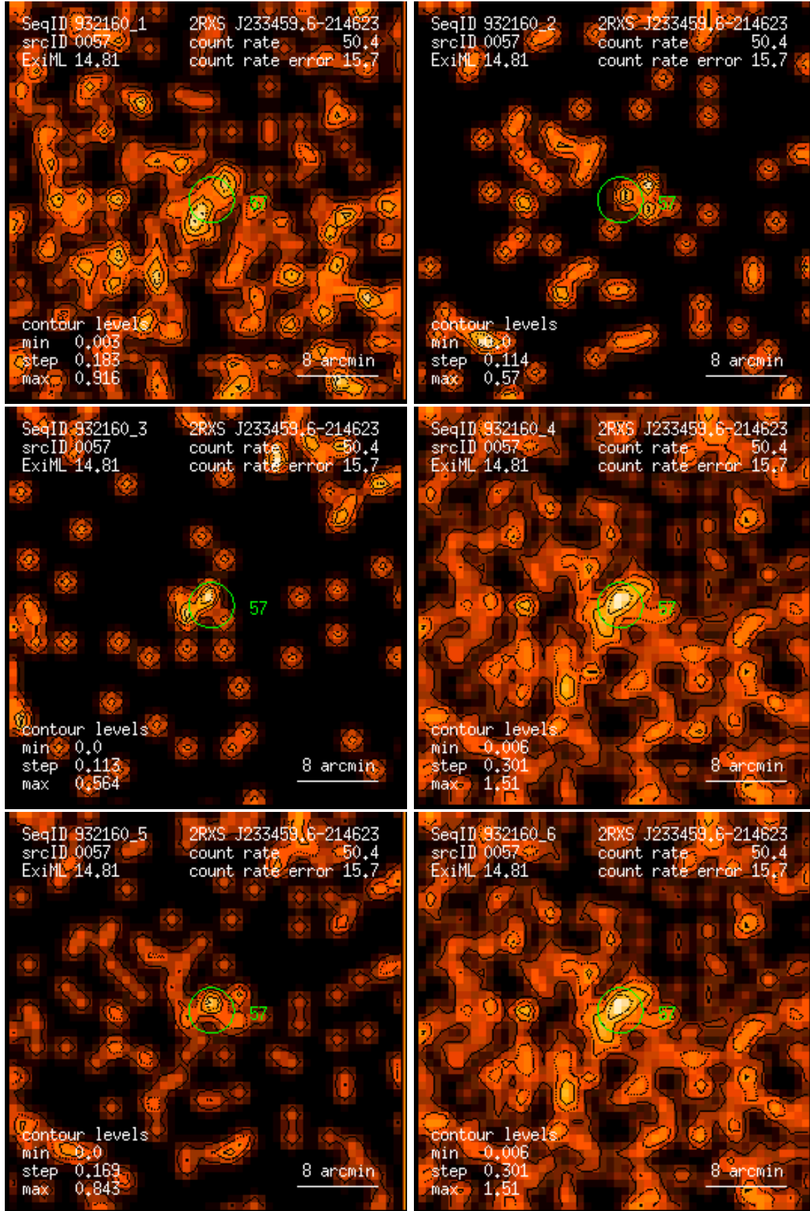
Figure 57: RASS 932160: detection 0057: band rate images, Gaussian filter: (1) PSPC channels 11 – 41, (2) 52 – 90, (3) 91 – 201, (4) 11 – 235, (5) 52 – 201, (6) 11 – 201. Broad band rates in counts/ks. Band rate contour levels in counts/ks/arcmin 2 .
