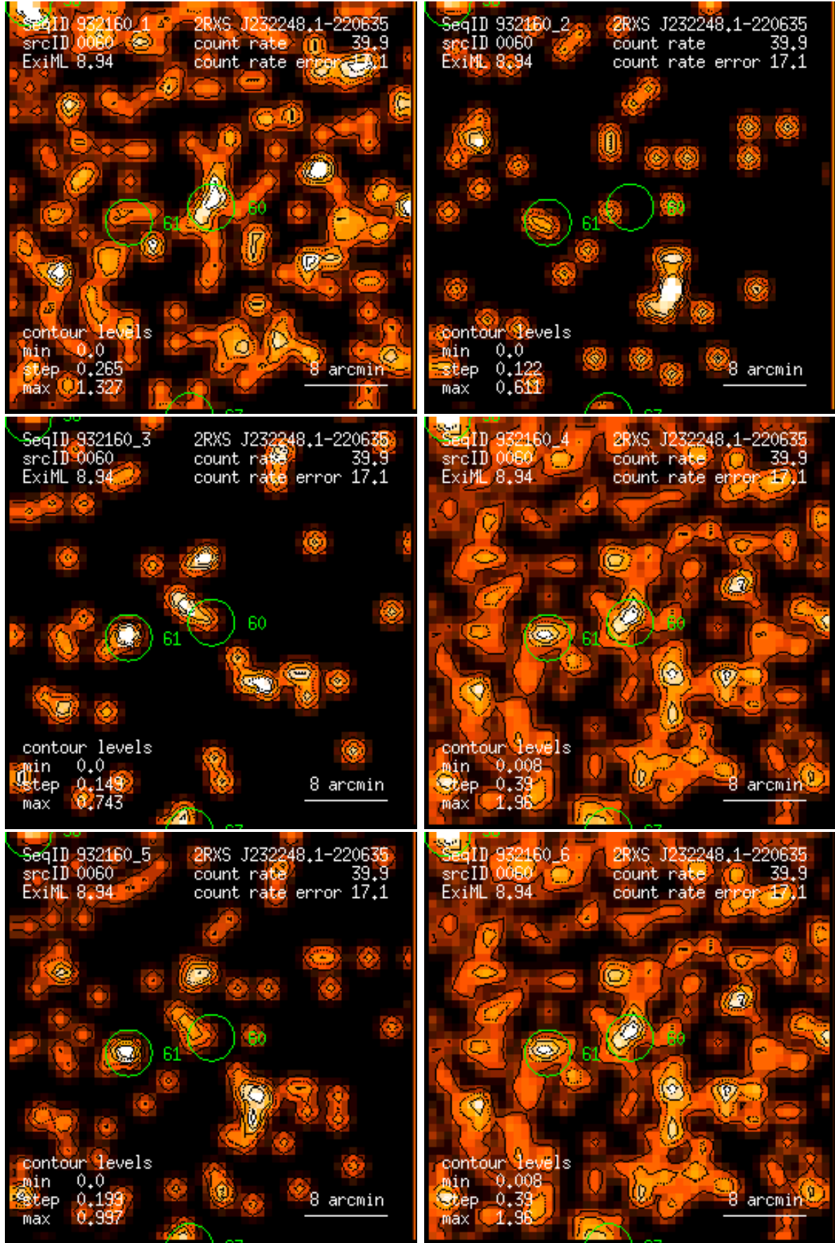
Figure 60: RASS 932160: detection 0060: band rate images, Gaussian filter: (1) PSPC channels 11 – 41, (2) 52 – 90, (3) 91 – 201, (4) 11 – 235, (5) 52 – 201, (6) 11 – 201. Broad band rates in counts/ks. Band rate contour levels in counts/ks/arcmin 2 .
