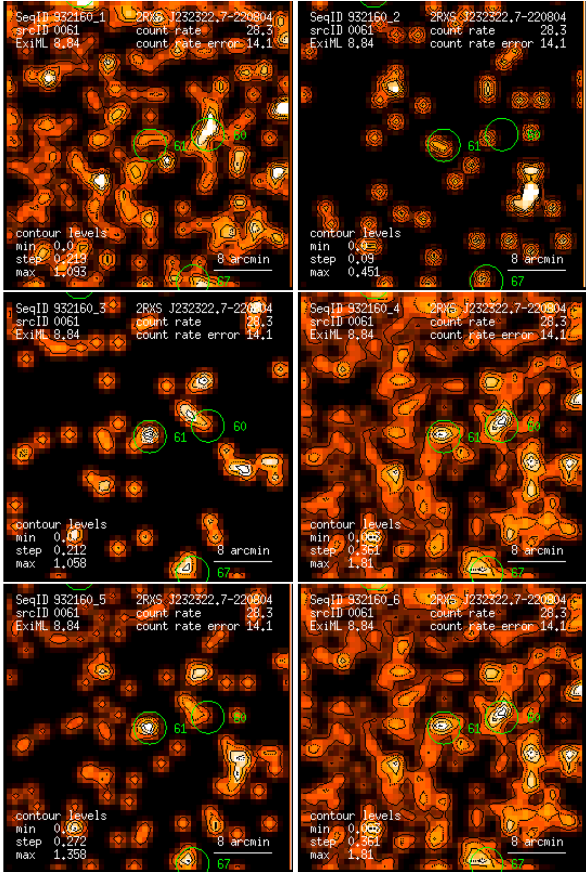
Figure 61: RASS 932160: detection 0061: band rate images, Gaussian filter: (1) PSPC channels 11 – 41, (2) 52 – 90, (3) 91 – 201, (4) 11 – 235, (5) 52 – 201, (6) 11 – 201. Broad band rates in counts/ks. Band rate contour levels in counts/ks/arcmin 2 .
