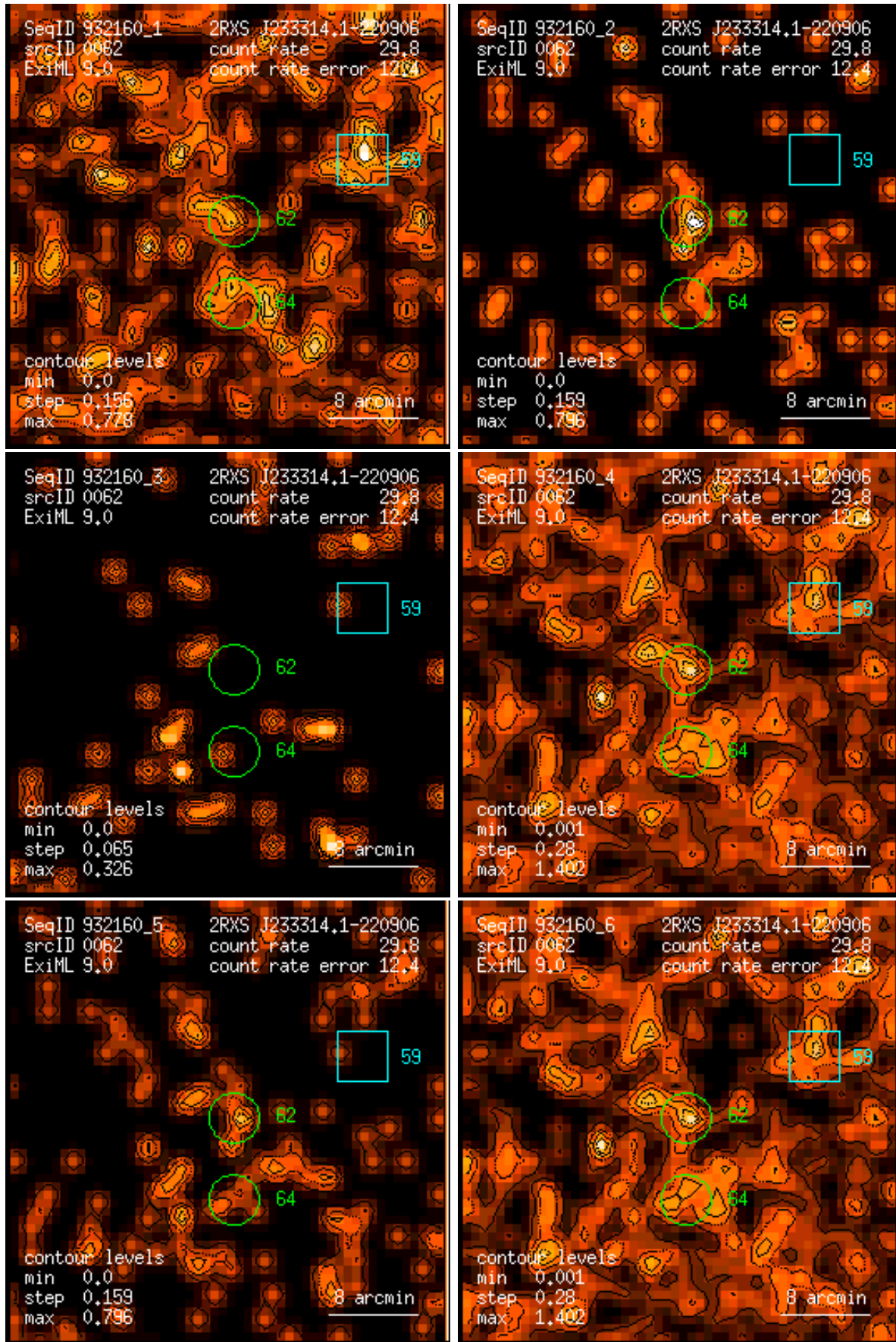
Figure 62: RASS 932160: detection 0062: band rate images, Gaussian filter: (1) PSPC channels 11 – 41, (2) 52 – 90, (3) 91 – 201, (4) 11 – 235, (5) 52 – 201, (6) 11 – 201. Broad band rates in counts/ks. Band rate contour levels in counts/ks/arcmin 2 .
