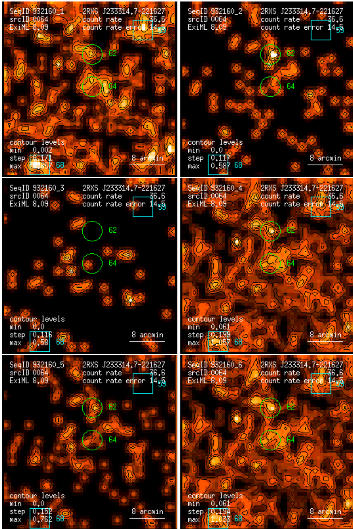
Figure 64: RASS 932160: detection 0064: band rate images, Gaussian filter: (1) PSPC channels 11 – 41, (2) 52 – 90, (3) 91 – 201, (4) 11 – 235, (5) 52 – 201, (6) 11 – 201. Broad band rates in counts/ks. Band rate contour levels in counts/ks/arcmin 2 .
