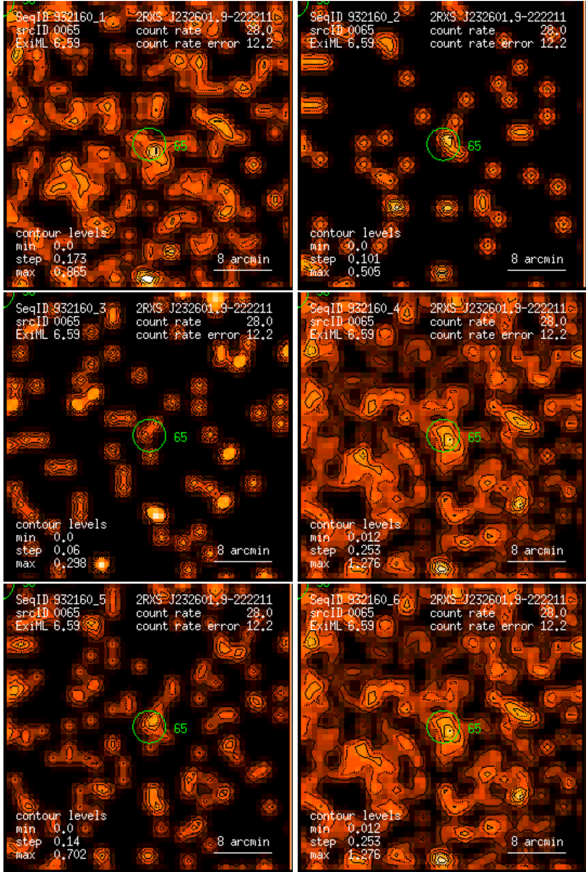
Figure 65: RASS 932160: detection 0065: band rate images, Gaussian filter: (1) PSPC channels 11 – 41, (2) 52 – 90, (3) 91 – 201, (4) 11 – 235, (5) 52 – 201, (6) 11 – 201. Broad band rates in counts/ks. Band rate contour levels in counts/ks/arcmin 2 .
