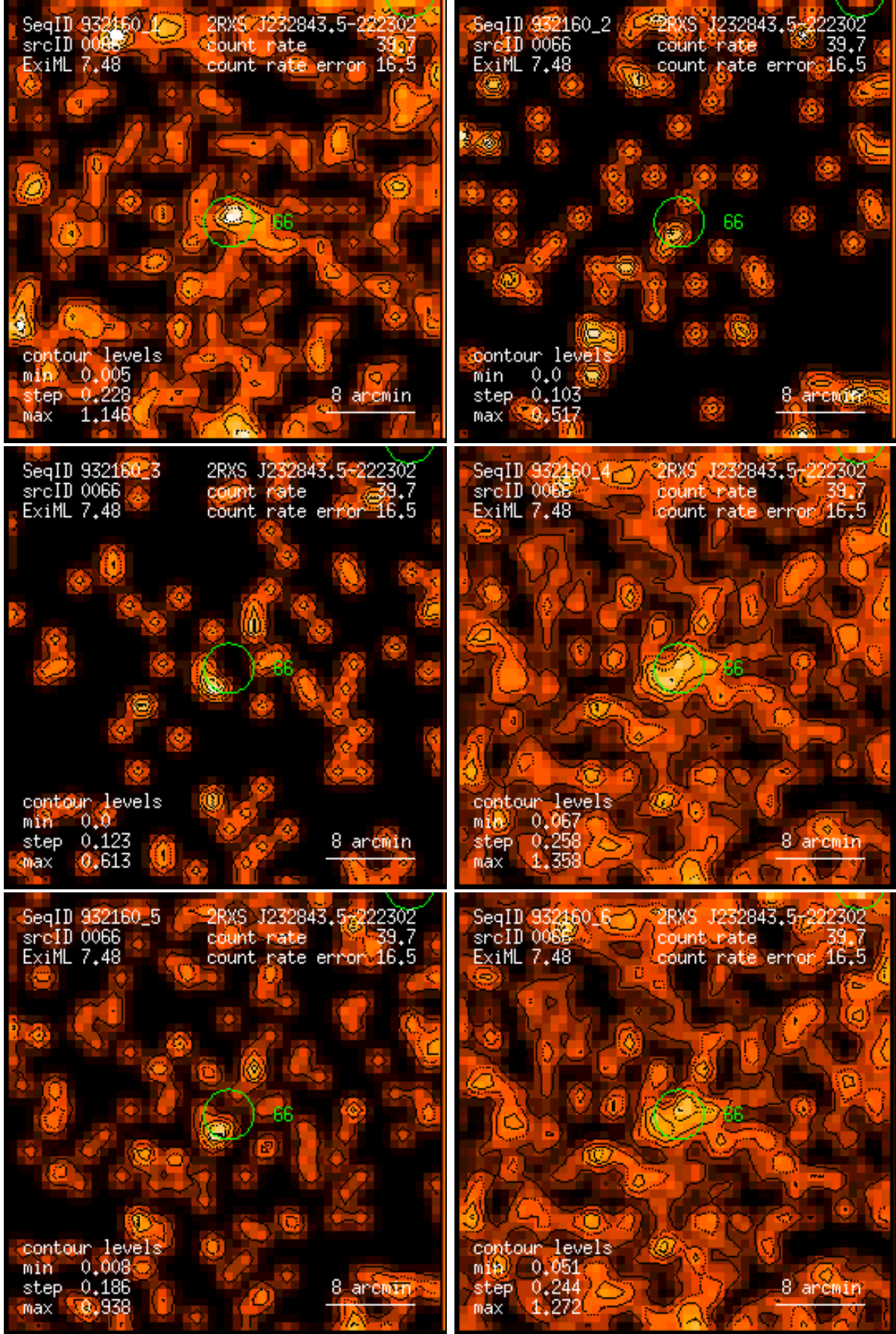
Figure 66: RASS 932160: detection 0066: band rate images, Gaussian filter: (1) PSPC channels 11 – 41, (2) 52 – 90, (3) 91 – 201, (4) 11 – 235, (5) 52 – 201, (6) 11 – 201. Broad band rates in counts/ks. Band rate contour levels in counts/ks/arcmin 2 .
