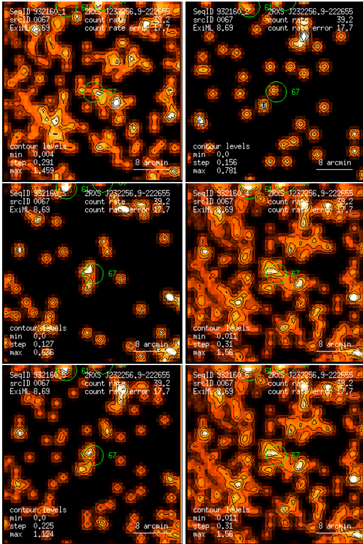
Figure 67: RASS 932160: detection 0067: band rate images, Gaussian filter: (1) PSPC channels 11 – 41, (2) 52 – 90, (3) 91 – 201, (4) 11 – 235, (5) 52 – 201, (6) 11 – 201. Broad band rates in counts/ks. Band rate contour levels in counts/ks/arcmin 2 .
