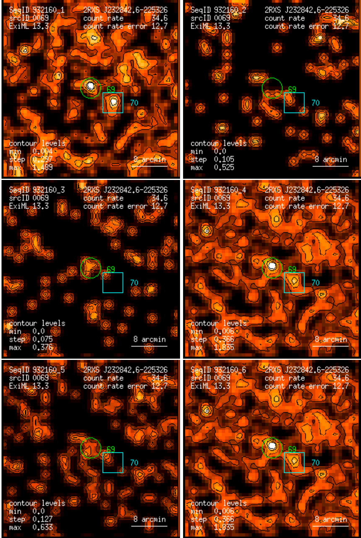
Figure 69: RASS 932160: detection 0069: band rate images, Gaussian filter: (1) PSPC channels 11 – 41, (2) 52 – 90, (3) 91 – 201, (4) 11 – 235, (5) 52 – 201, (6) 11 – 201. Broad band rates in counts/ks. Band rate contour levels in counts/ks/arcmin 2 .
