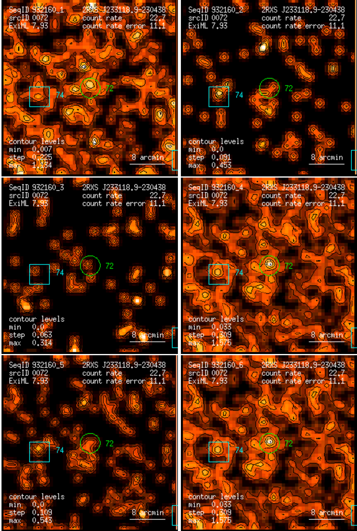
Figure 72: RASS 932160: detection 0072: band rate images, Gaussian filter: (1) PSPC channels 11 – 41, (2) 52 – 90, (3) 91 – 201, (4) 11 – 235, (5) 52 – 201, (6) 11 – 201. Broad band rates in counts/ks. Band rate contour levels in counts/ks/arcmin 2 .
