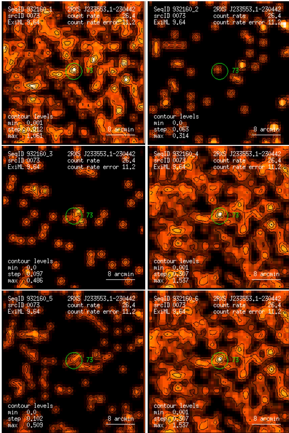
Figure 73: RASS 932160: detection 0073: band rate images, Gaussian filter: (1) PSPC channels 11 – 41, (2) 52 – 90, (3) 91 – 201, (4) 11 – 235, (5) 52 – 201, (6) 11 – 201. Broad band rates in counts/ks. Band rate contour levels in counts/ks/arcmin 2 .
