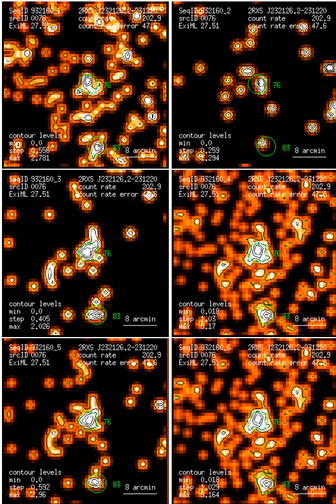
Figure 76: RASS 932160: detection 0076: band rate images, Gaussian filter: (1) PSPC channels 11 – 41, (2) 52 – 90, (3) 91 – 201, (4) 11 – 235, (5) 52 – 201, (6) 11 – 201. Broad band rates in counts/ks. Band rate contour levels in counts/ks/arcmin 2 .
