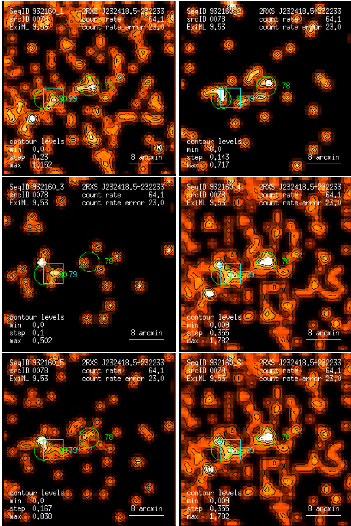
Figure 78: RASS 932160: detection 0078: band rate images, Gaussian filter: (1) PSPC channels 11 – 41, (2) 52 – 90, (3) 91 – 201, (4) 11 – 235, (5) 52 – 201, (6) 11 – 201. Broad band rates in counts/ks. Band rate contour levels in counts/ks/arcmin 2 .
