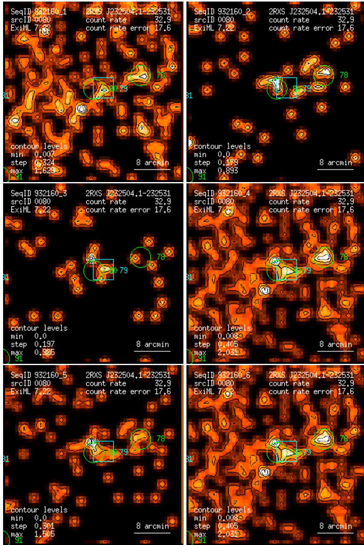
Figure 80: RASS 932160: detection 0080: band rate images, Gaussian filter: (1) PSPC channels 11 – 41, (2) 52 – 90, (3) 91 – 201, (4) 11 – 235, (5) 52 – 201, (6) 11 – 201. Broad band rates in counts/ks. Band rate contour levels in counts/ks/arcmin 2 .
