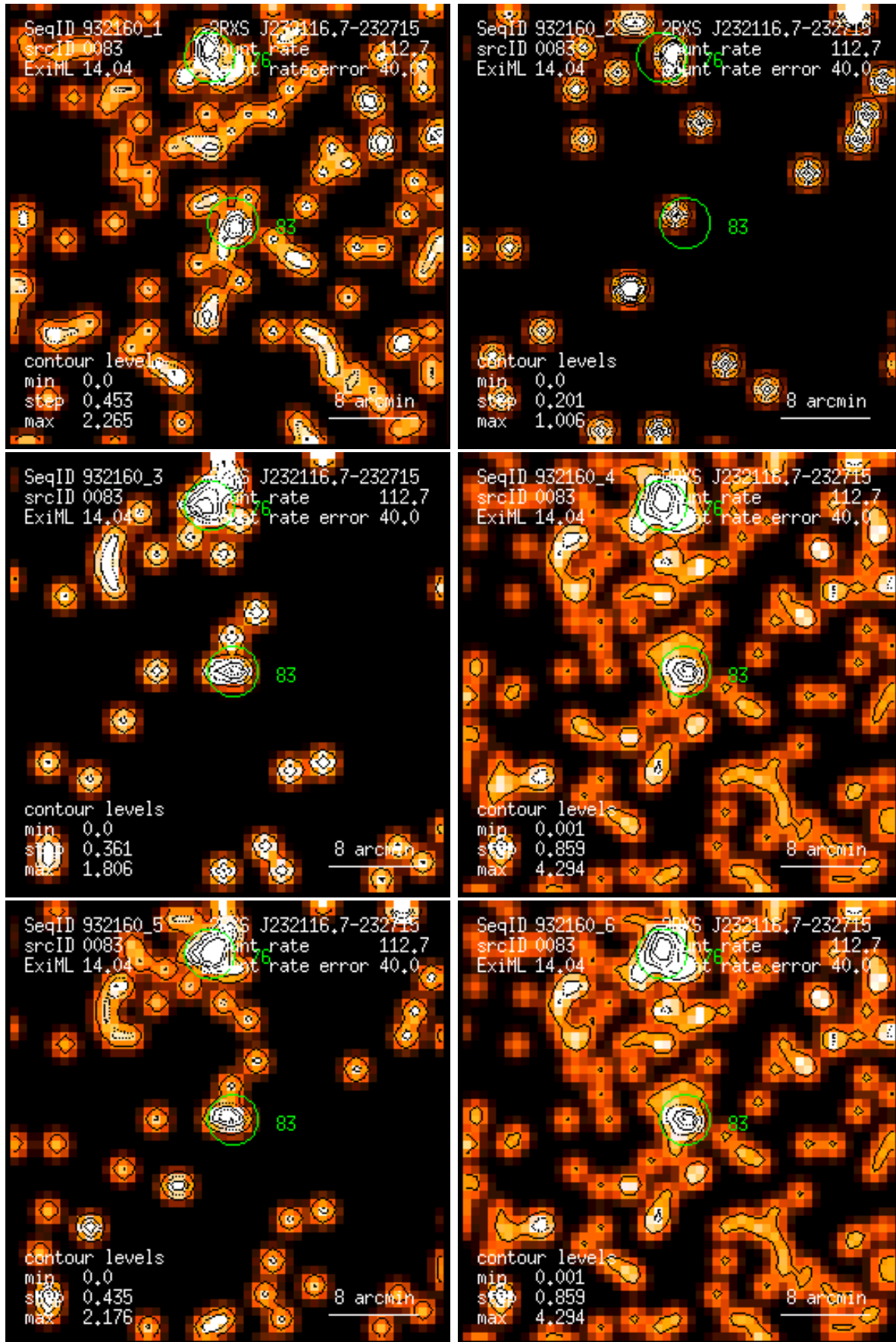
Figure 83: RASS 932160: detection 0083: band rate images, Gaussian filter: (1) PSPC channels 11 – 41, (2) 52 – 90, (3) 91 – 201, (4) 11 – 235, (5) 52 – 201, (6) 11 – 201. Broad band rates in counts/ks. Band rate contour levels in counts/ks/arcmin 2 .
