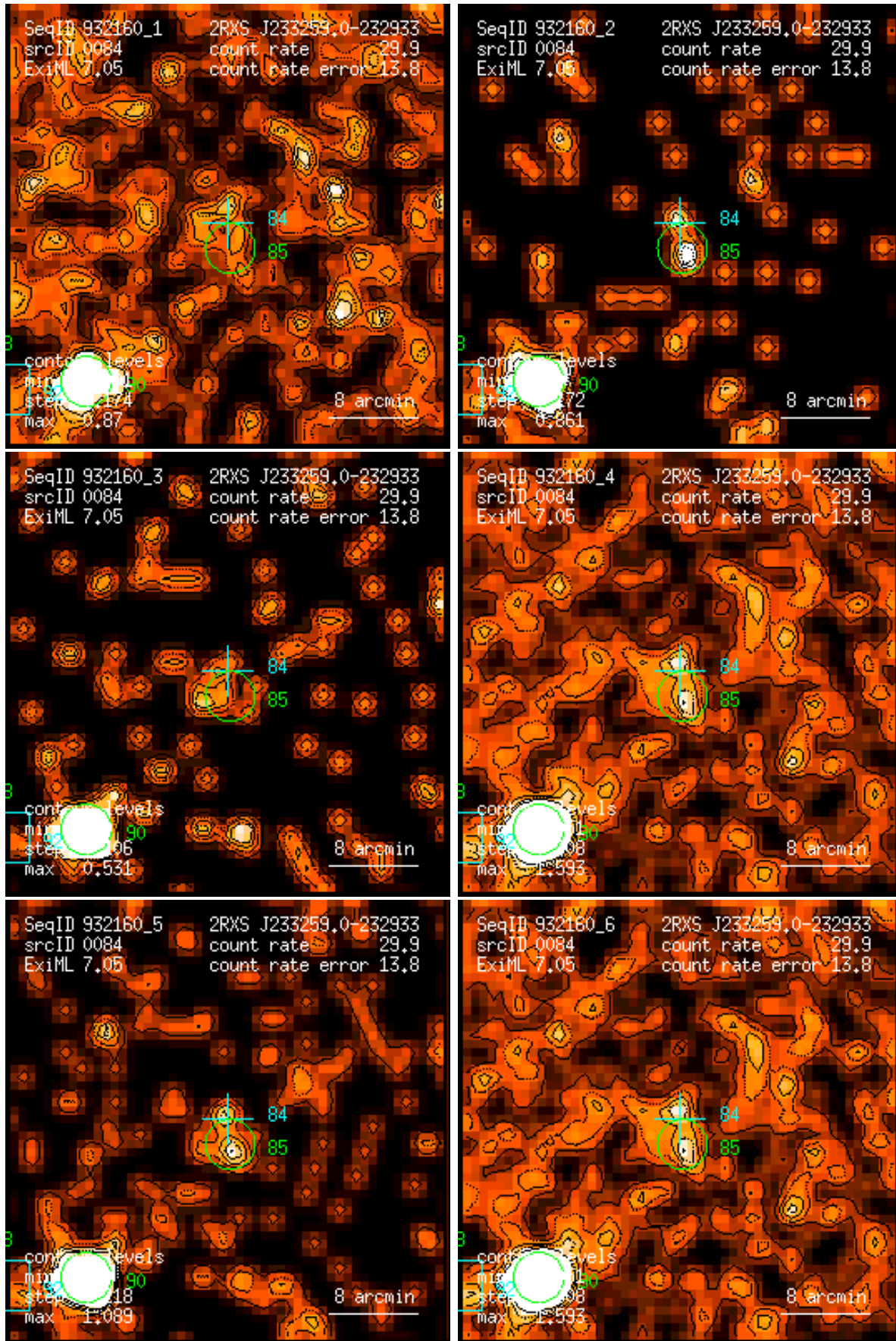
Figure 84: RASS 932160: detection 0084: band rate images, Gaussian filter: (1) PSPC channels 11 – 41, (2) 52 – 90, (3) 91 – 201, (4) 11 – 235, (5) 52 – 201, (6) 11 – 201. Broad band rates in counts/ks. Band rate contour levels in counts/ks/arcmin 2 .
