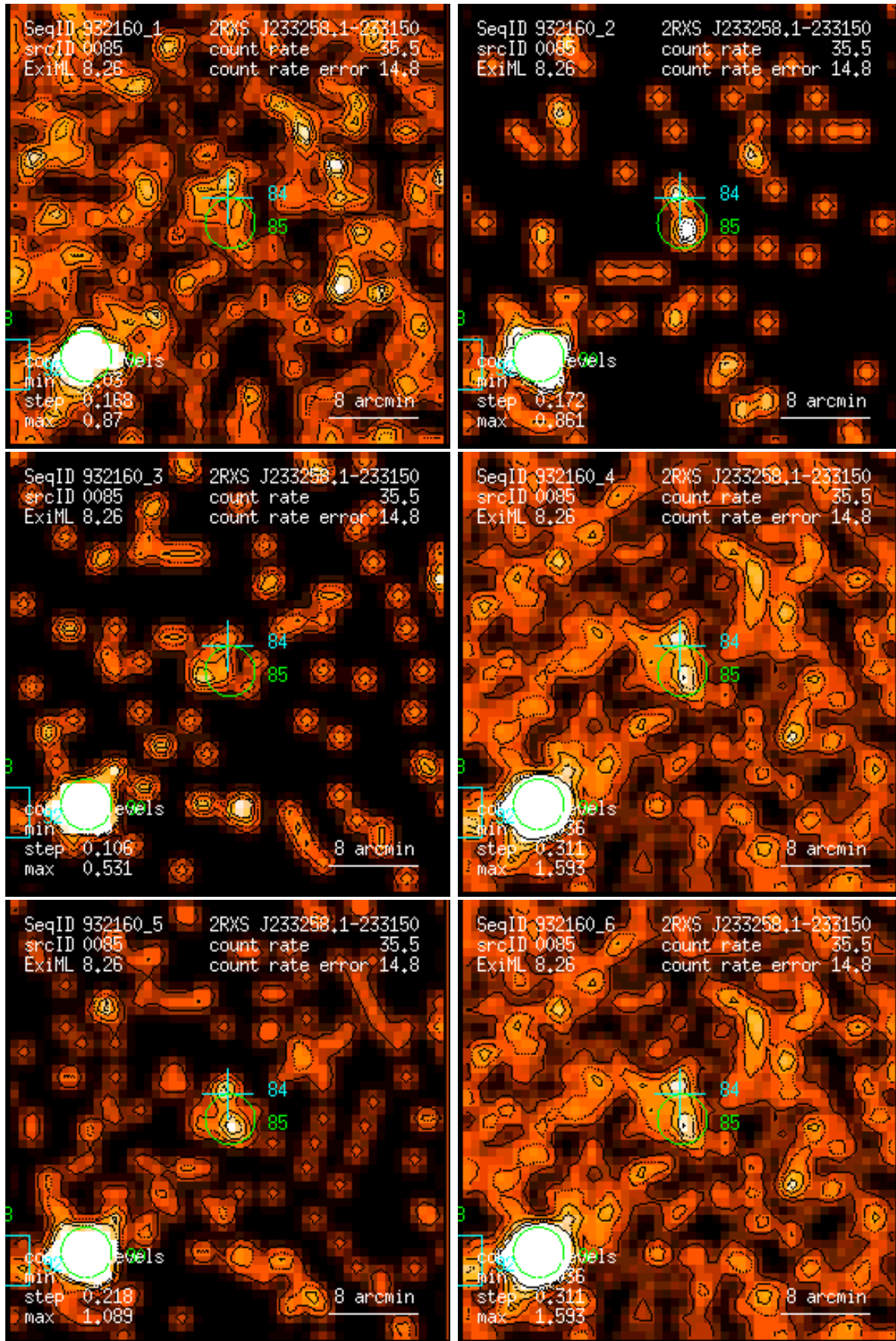
Figure 85: RASS 932160: detection 0085: band rate images, Gaussian filter: (1) PSPC channels 11 – 41, (2) 52 – 90, (3) 91 – 201, (4) 11 – 235, (5) 52 – 201, (6) 11 – 201. Broad band rates in counts/ks. Band rate contour levels in counts/ks/arcmin 2 .
