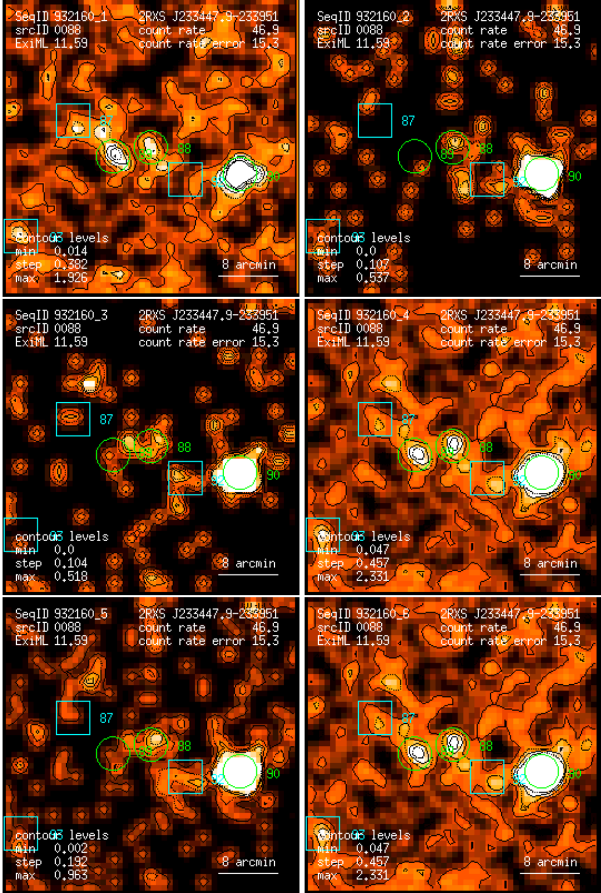
Figure 88: RASS 932160: detection 0088: band rate images, Gaussian filter: (1) PSPC channels 11 – 41, (2) 52 – 90, (3) 91 – 201, (4) 11 – 235, (5) 52 – 201, (6) 11 – 201. Broad band rates in counts/ks. Band rate contour levels in counts/ks/arcmin 2 .
